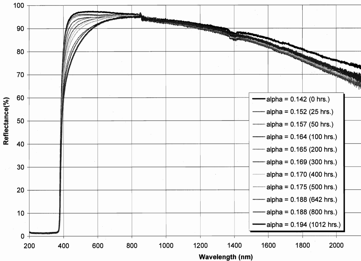
Figure A16. Spectral Reflectance History of Specimen I4: Zinvisible K Formula 3 AQ-20 (C-762/CH-18)
