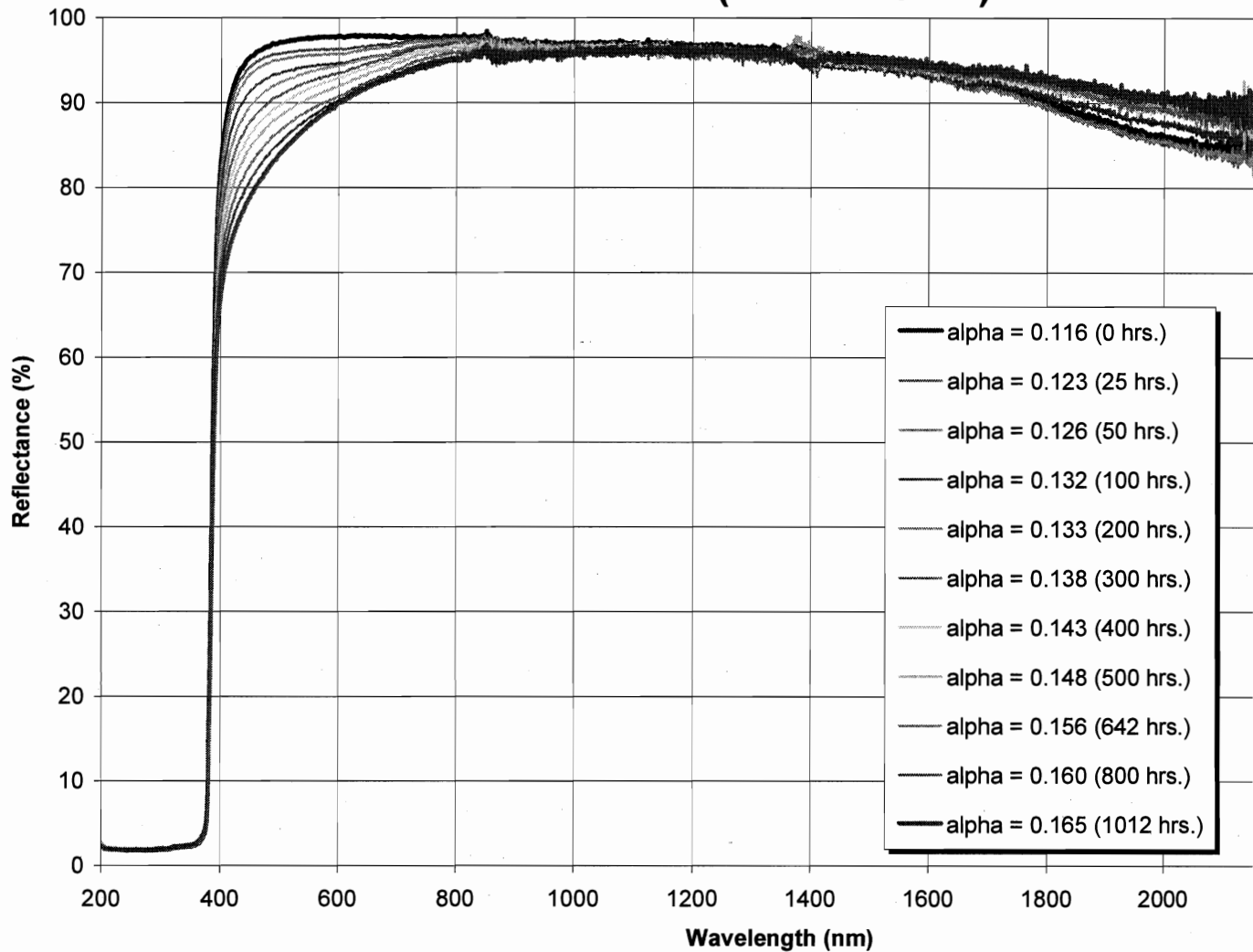
Figure A19. Spectral Reflectance History of Specimen C: Z-93P (C-759/CG-21)
