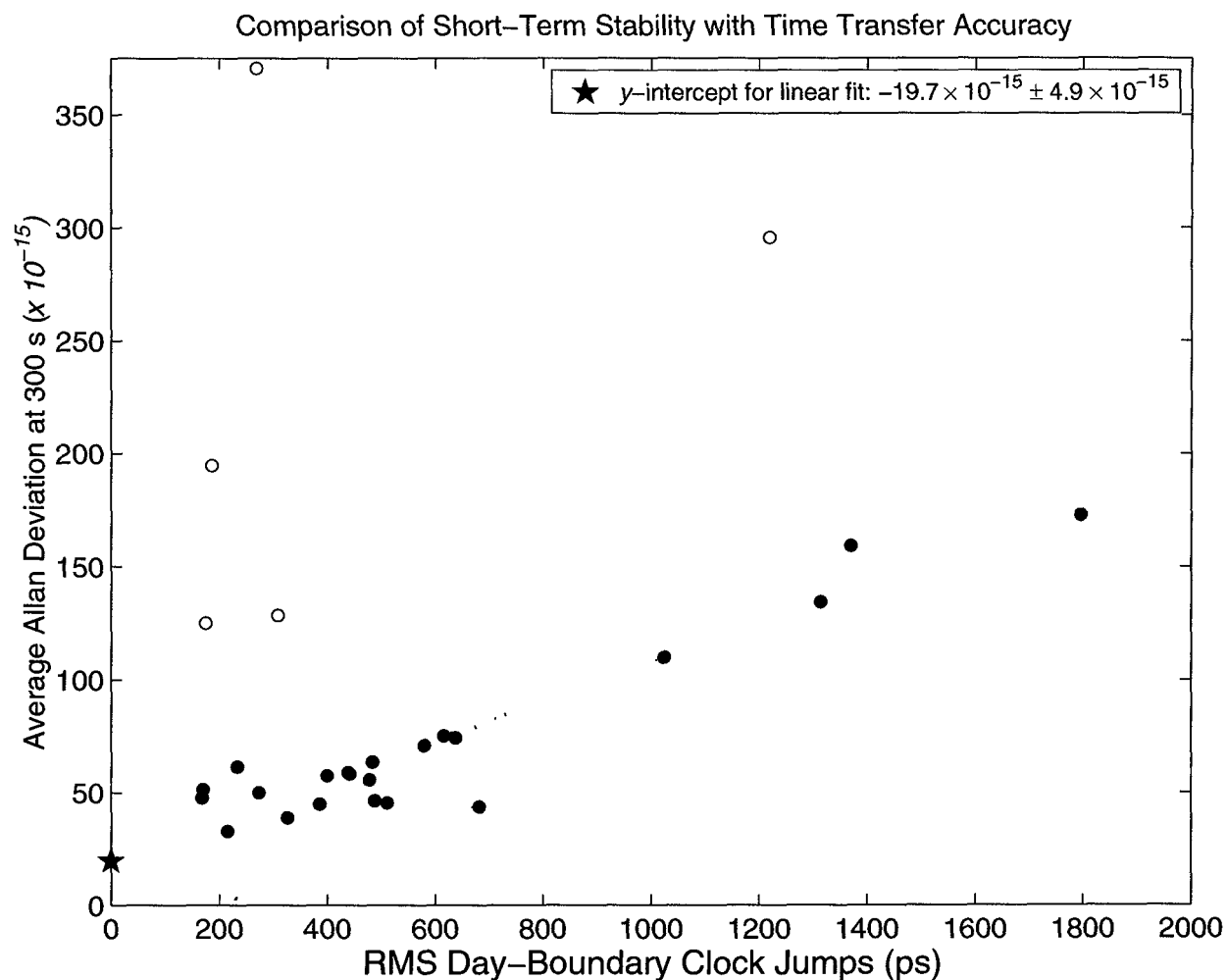
Figure 6: The average Allan deviations computed at 300-s intervals versus the RMS day-boundary clock discontinuities for all stations. Two connected points are shown for each of the stations ALGO, HOB2, MATE, and NRC1, for the intervals given in Table 1. The stations with local timing instabilities (ONSA, TIDB, CRO1, IRKT, and METS, indicated by open circles) are not included in the linear fit for the general trend.
