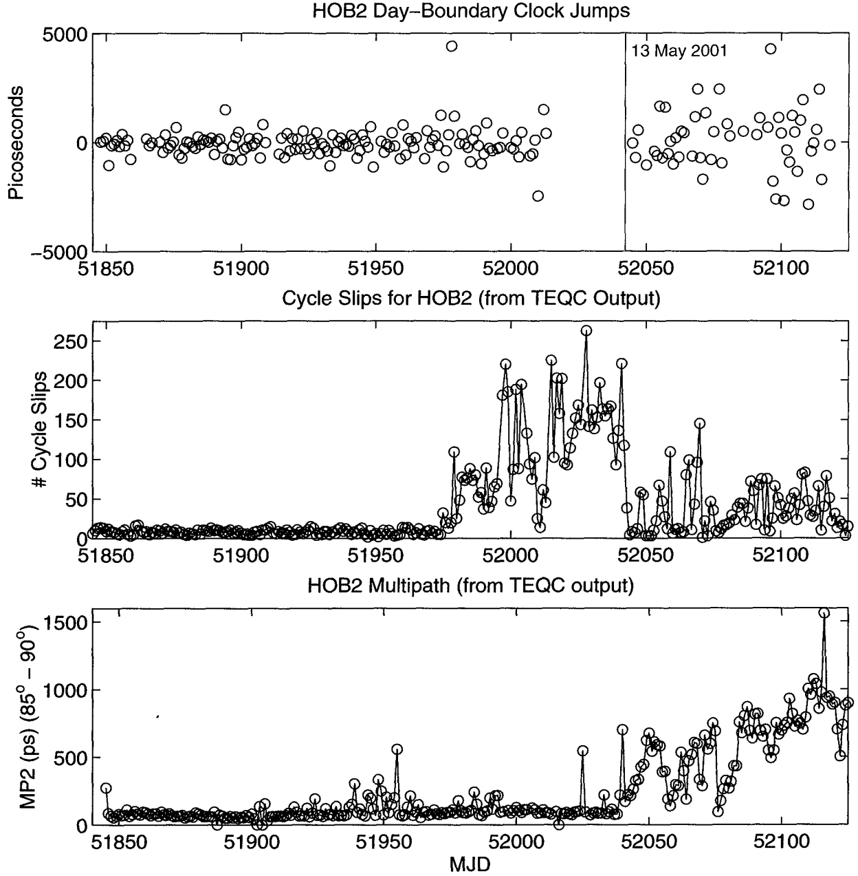
Figure 5: Time series of results for HOB2 (Hobert, Australia). Upper panel (a) shows the raw day-boundary clock discontinuities illustrating the large increase in variations after 13 May 2001. Middle panel (b) shows the daily number of carrier phase cycle slips as reported by the quality-checking utility TEQC. Lower panel (c) shows the TEQC multipath index MP2 for observations in the elevation angle bin from 85^\circ to 90^\circ .
