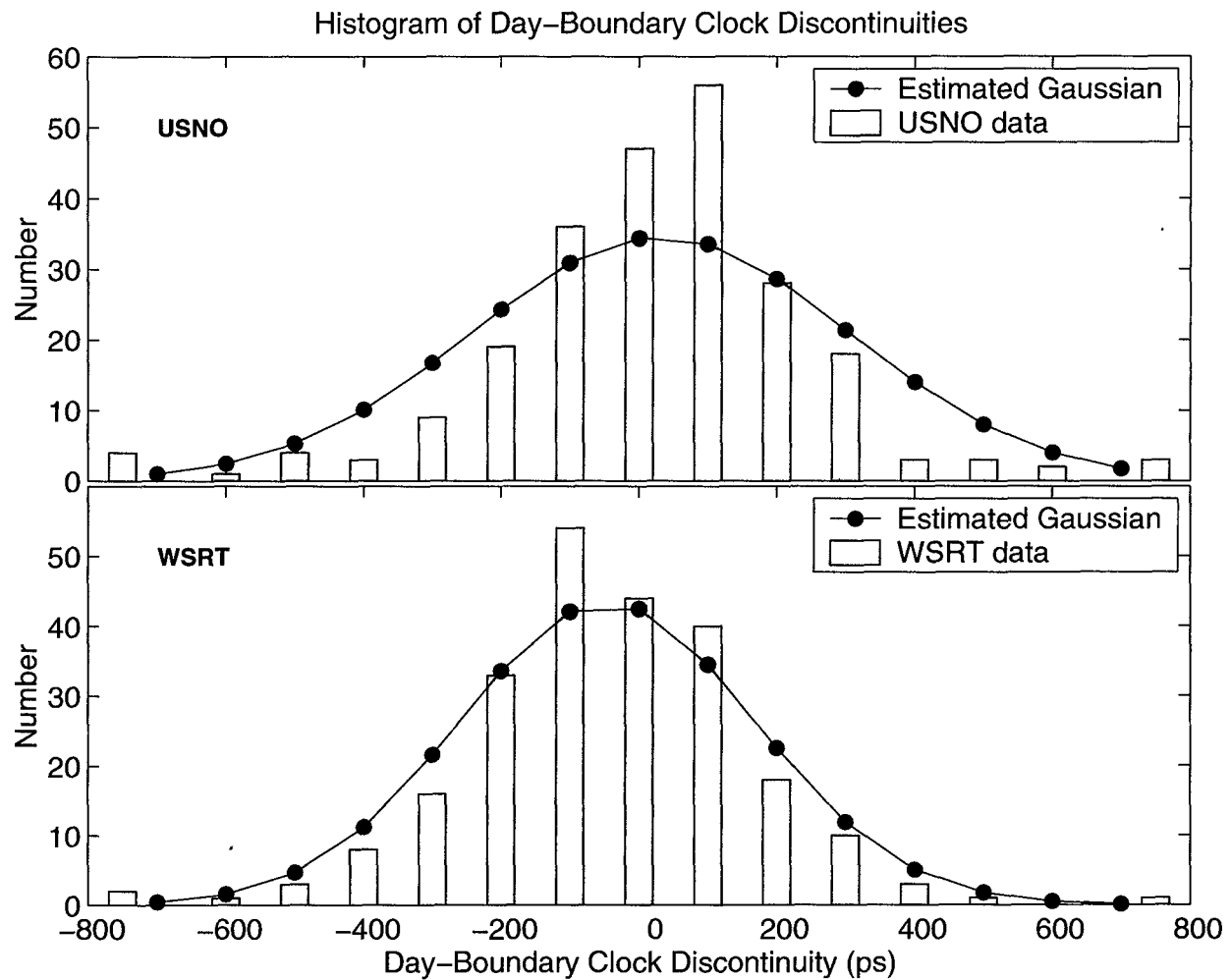
Figure 4: Histograms of the day-boundary clock discontinuities for USNO and WSRT compared with Gaussian distributions for each.
