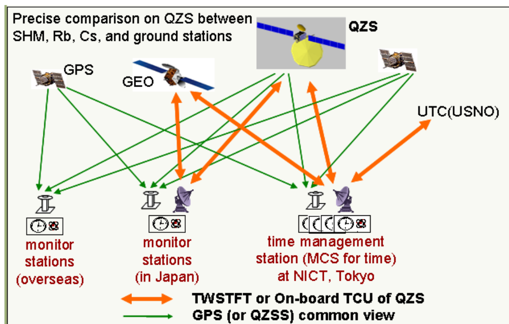
Figure 13. Basic design of QZS time management system.
