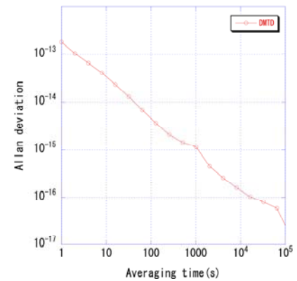
Figure 7. System noise of the multi-channel DMTD.
