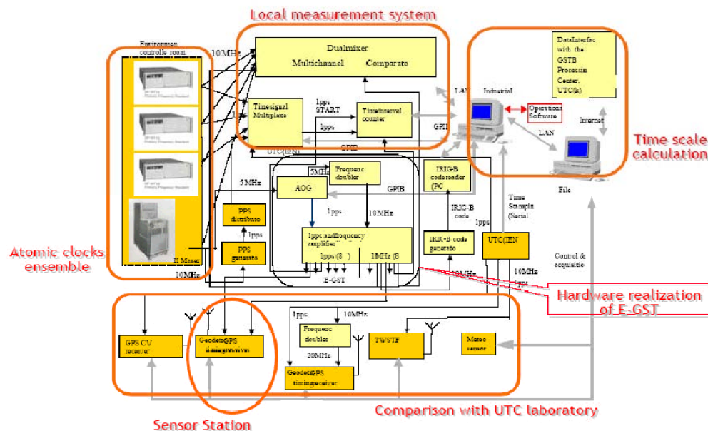
Figure 1. The E-PTS architecture and its major functions.
