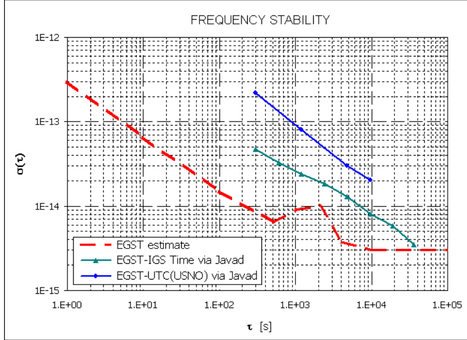
Figure 9. E-GST frequency stability as estimated versus the IGS time scale by a Precise Point Positioning (PPP) technique (green line) and versus UTC (USNO) by OD&TS processing (blue line). The E-GST stability as measured inside the E-PTS is also reported (dashed red line) as a reference.
