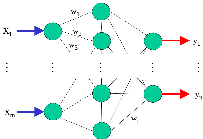
Figure 2: Neural Nets
