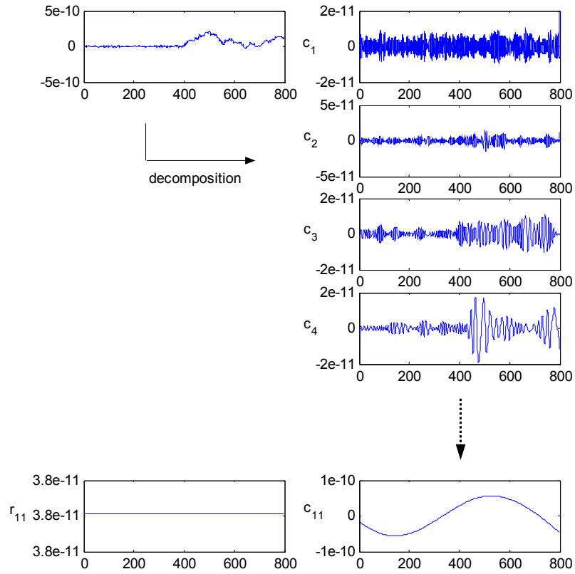
Figure 9. IMF components of the concatenated noise.
