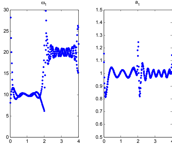
Figure 4. The instantaneous frequencies and amplitudes of IMFs in s_2(t) .
