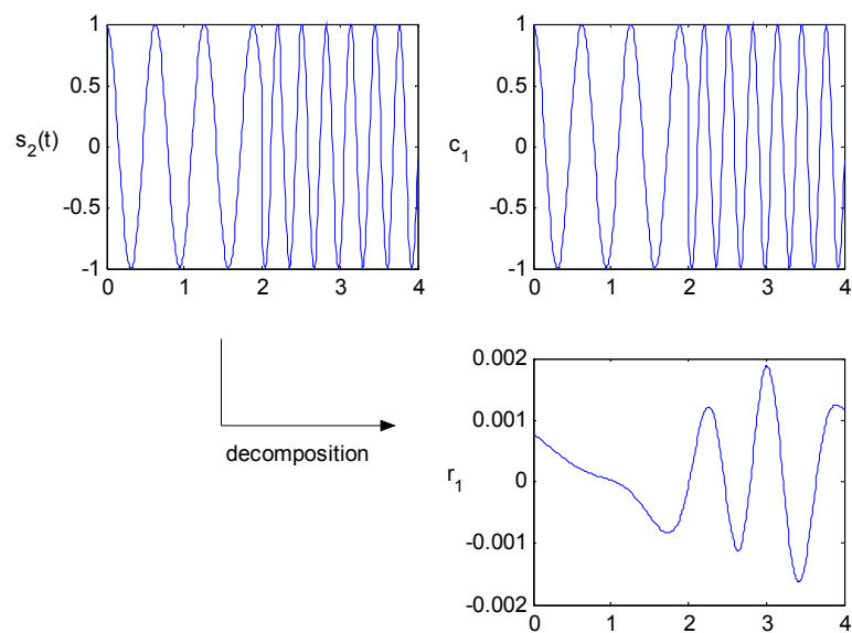
Figure 3. s_2(t) and its corresponding IMF components.
