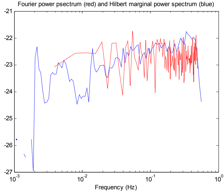
Figure 6. Marginal spectrum and power spectrum for white phase modulation noise.
