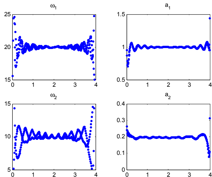
Figure 2. The instantaneous frequencies and amplitudes of IMFs in s_1(t) .
