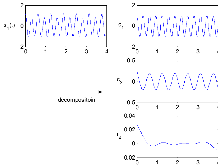
Figure 1. s_1(t) and its corresponding IMF components.
