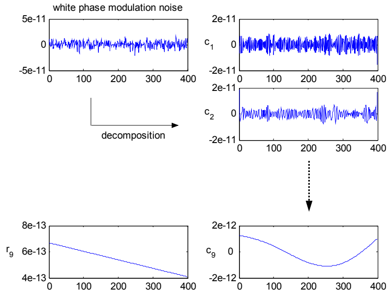
Figure 5. White phase modulation noise and its IMF components.
