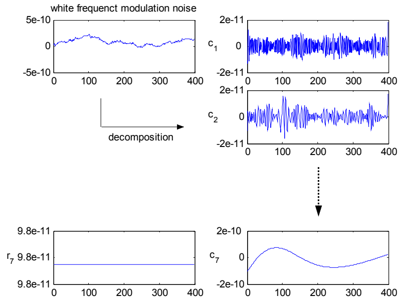
Figure 7. White frequency modulation noise and its IMF components.
