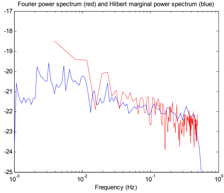
Figure 8. Marginal spectrum and power spectrum for white frequency modulation noise.
