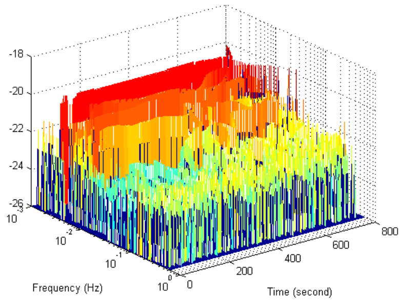
Figure 10. Hilbert power spectrum for the concatenated noise.
