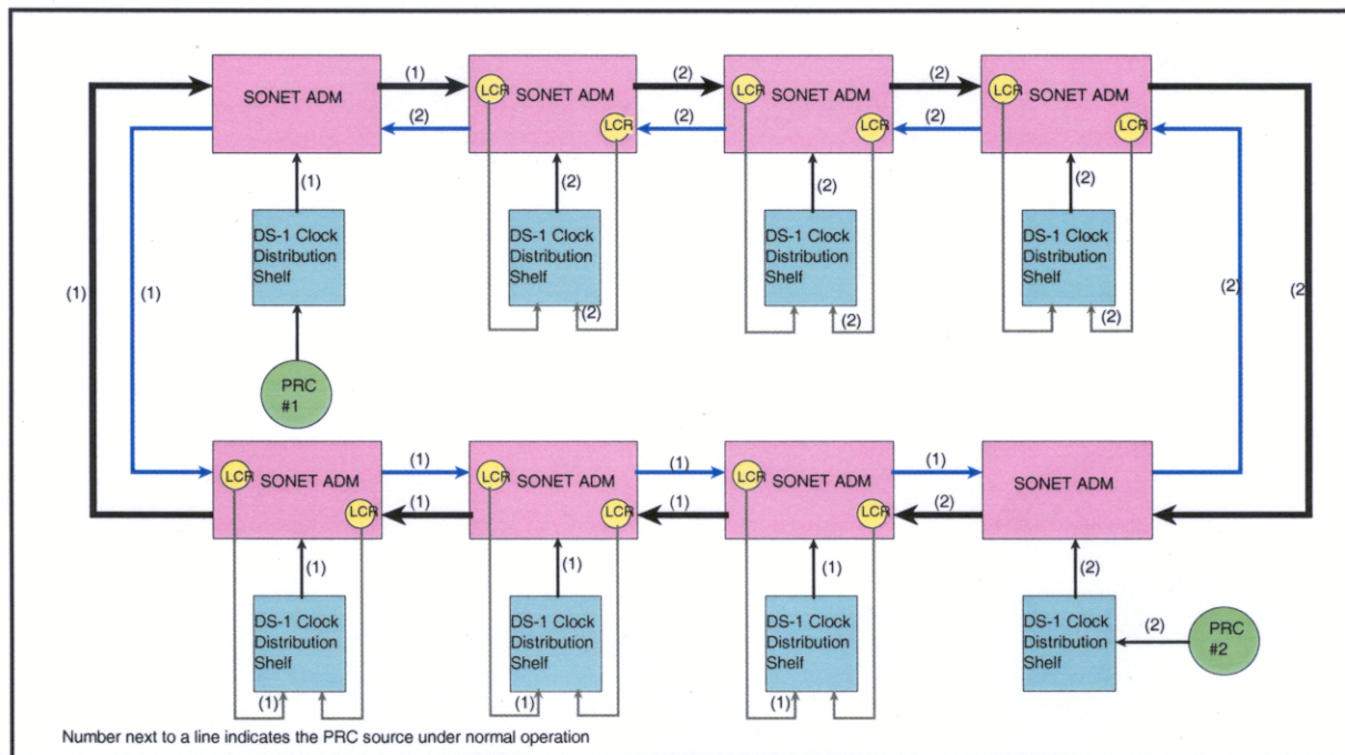
Figure 11: Timing in SONET Ring Using Recovered Optical Line Timing.
