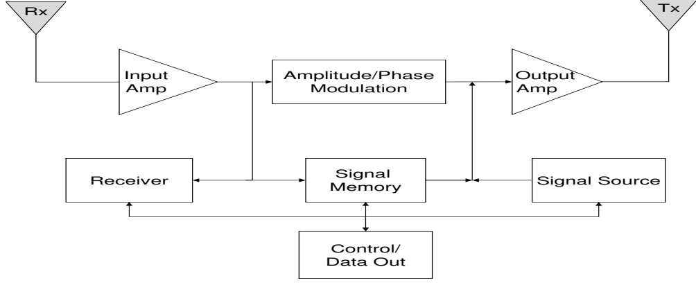
Figure 4.1: Repeater jammer block diagram [26].
