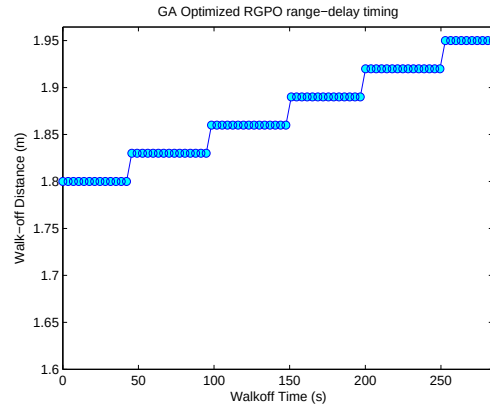
(b) Optimized RGPO Range-Delay Profile.
