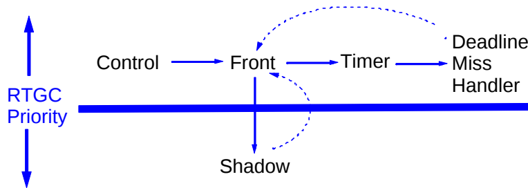
Figure 2. Interaction Among the Participants
