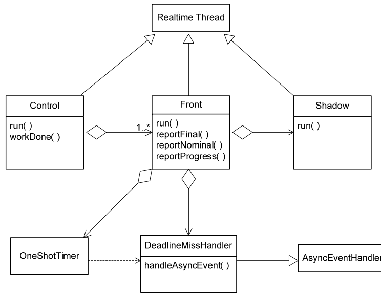
Figure 1. Participants of the Shadow Design Pattern
