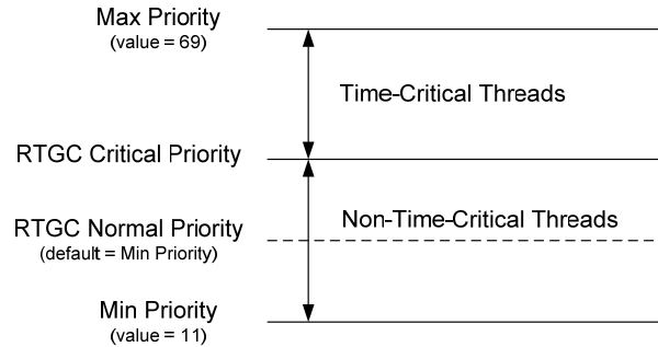
Figure 3. Classification of thread priorities
