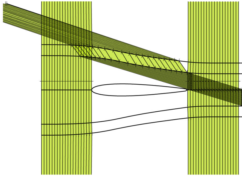
Figure 15: Wall shape design using ray-tracing technique
