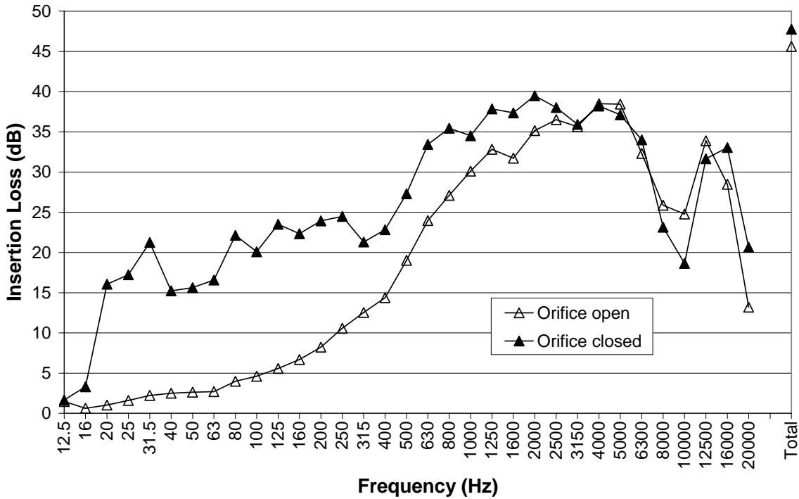
Figure 4 Insertion loss measurements for the Surefire EP3 Sonic Defender™.
