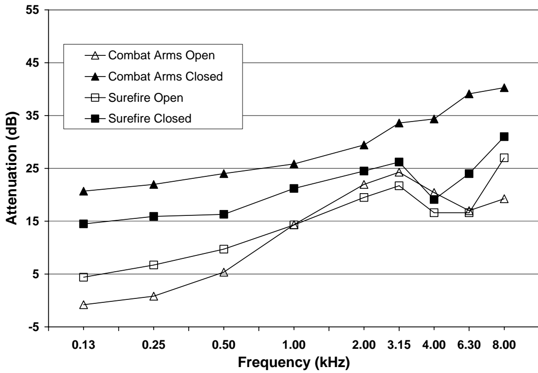
Figure 5 A comparison of results: the Surefire EP3 Sonic Defender™ versus the E-A-R® Combat Arms earplug.
