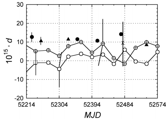
Figure 3. Fractional deviation d of the duration of the TAI scale interval from the SI second as realized by the individual primary clocks CSF1 (●), CS1 (O) and CS2 (⊕) of PTB, NIST-F1 (▲), CRL-01 (X) (Japan), and JPO (□) (BNM-SYRTE, France) during the period MJD 52214-52574. MJD designates the Modified Julian Date; MJD 52574 corresponds to 2002 October 27. Data points from PTB's primary clocks were connected, as these clocks were operated continuously. Other symbols were plotted at the end of the measurement interval of typically 20 days. Error bars (one representative for each clock) indicate the 1\sigma standard uncertainty in the determination of d (source: BIPM Circular T).
