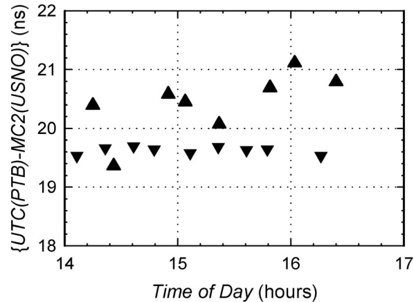
Figure 6. Time scale comparison UTC(PTB) - MC2(USNO) during the calibration experiment in PTB on MJD 52436, using a transportable X-band station (symbol ▲) and the standard KU-band TWSTFT equipment (symbol ▼), in operation out of the normal schedule. Each point represents an average over 2 minutes.
