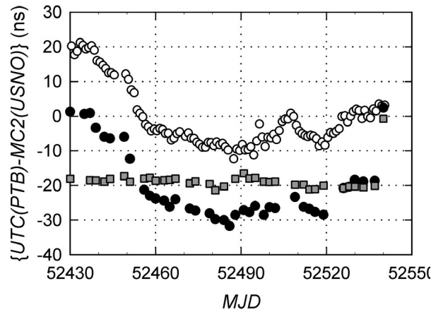
Figure 5. Results of a time scale comparison UTC(PTB) - MC2(USNO) using different techniques. X-band data (open circles) are daily averages over usually 22 to 24 15-minute session means. Ku-band data (full circles) are taken from standard ITU files. On MJD 52540, the CALR value in the header of the file reporting the TWSTFT results [11] in the ITU-format was changed due to the calibration experiment on MJD 52435, which explains the step in the Ku-band data and the differences (squares).
