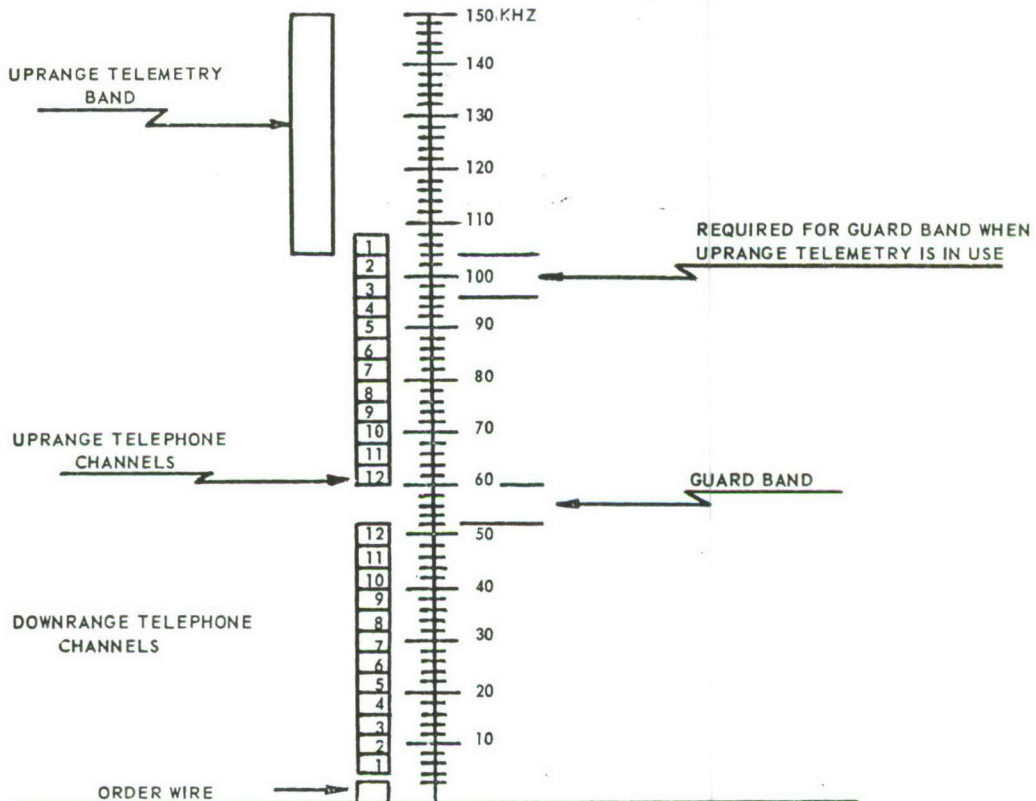
FIGURE 23 BANDWIDTH ALLOCATION - CAPE TO Eleuthera (W. E. CABLE)
