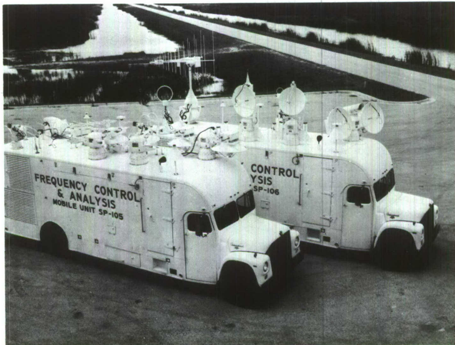
FCA VANS
