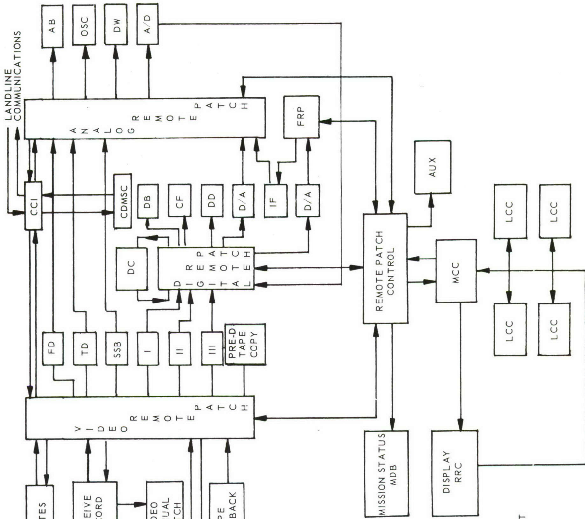
FIGURE 19, TEL 4 SYSTEMS BLOCK DIAGRAM
