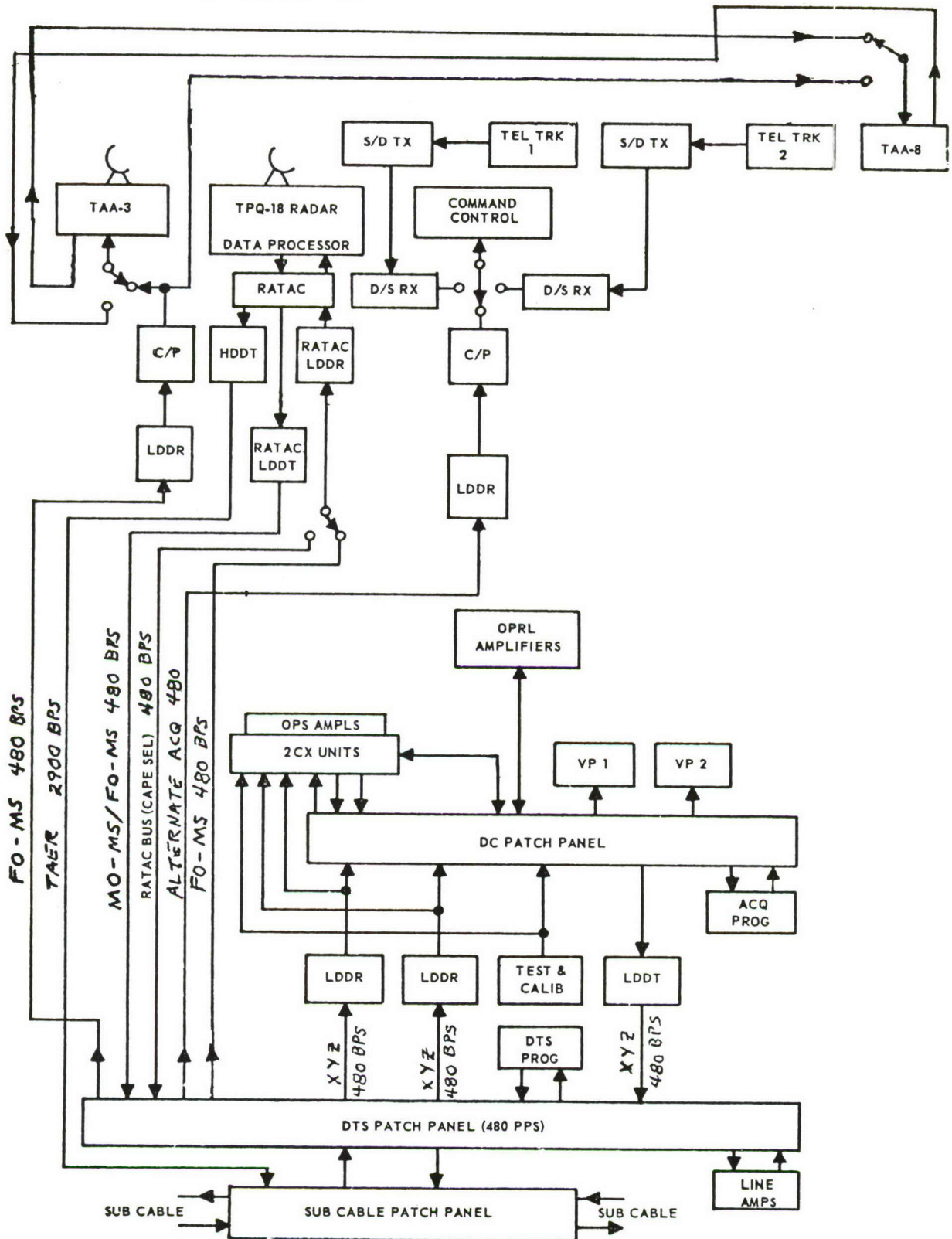
FIGURE 35 GRAND TURK ACQUISITION SYSTEM
