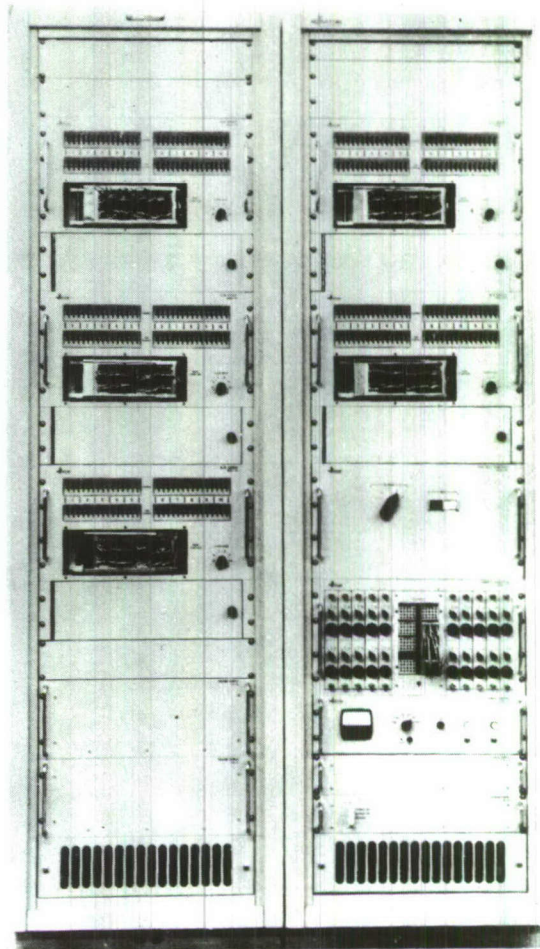
D/A CONVERTER
