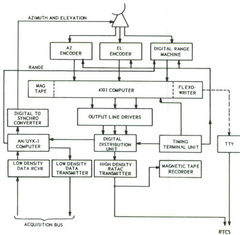
FIGURE 9 MIPIR ON-CABLE SITE DATA FLOW
