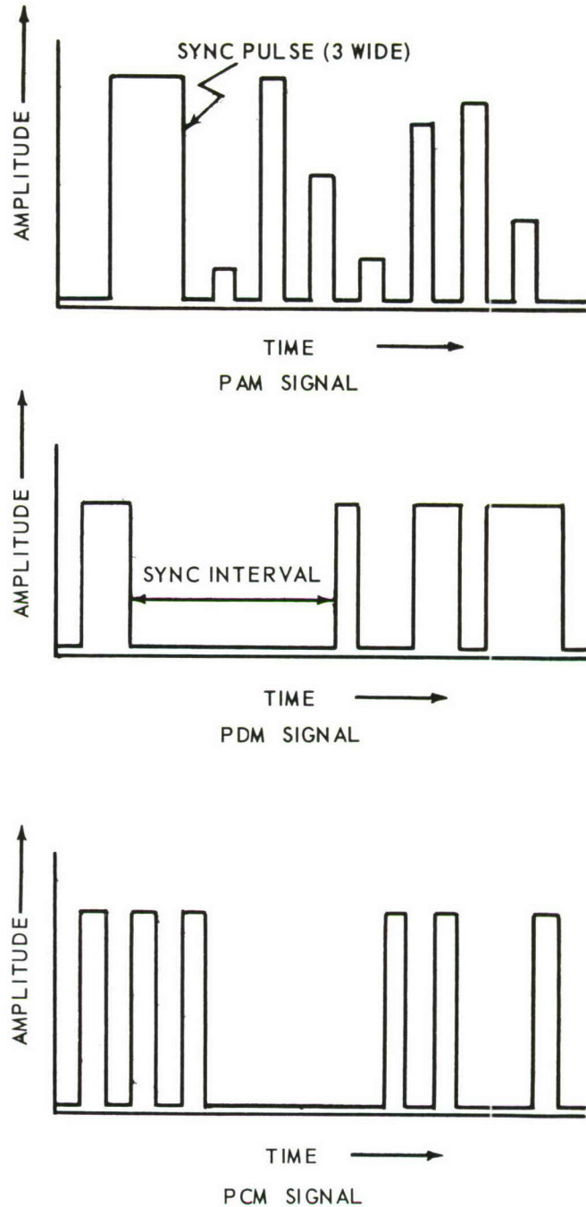
FIGURE 16 TYPICAL TDM WAVEFORMS
