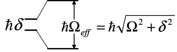
Figure 6. Two unshifted (left) and shifted (right) energy levels in the dressed-state picture. When \delta is positive, the ground state is the upper level.
