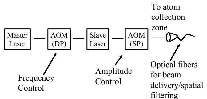
Figure 1. A master laser beam goes through a double pass AOM and injection locks a slave laser. The slave's beam goes through a single pass AOM for amplitude control before being coupled to a single mode fiber for delivery to the atoms. Either the double pass or the single pass AOM can be used to attenuate the resonant light as described in the text.
