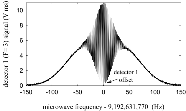
Figure 4. Raw data showing rapidly oscillating Ramsey fringes superimposed on a broader Rabi profile. Plotted are areas under the time-of-flight fluorescence signals (Fig. 3) as a function of applied microwave frequencies. No phase change is applied between the first and second pass through the Ramsey microwave cavity. Arrow indicates that some atoms do not participate in the oscillations and thus contribute to an offset.
