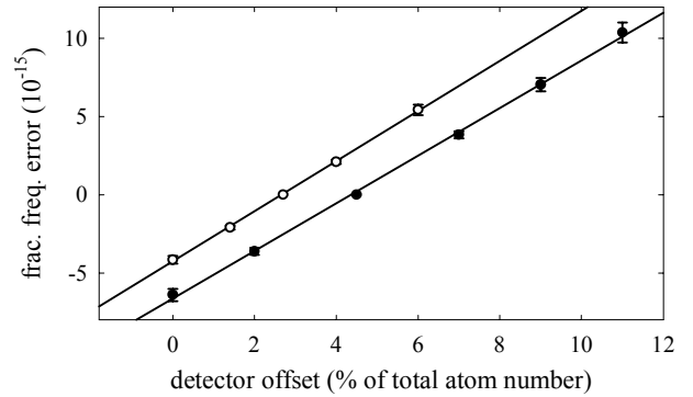
Figure 7. When analyzing clock data, different detector offset values lead to different deduced frequencies. Fractional frequency shifts as a function of detector offset are shown for detector 1 (filled circles) and detector 2 (unfilled circles). Linear regressions (lines) give y = 1.5x - 6.6 for detector 1 and y = 1.6x - 4.3 for detector 2.
