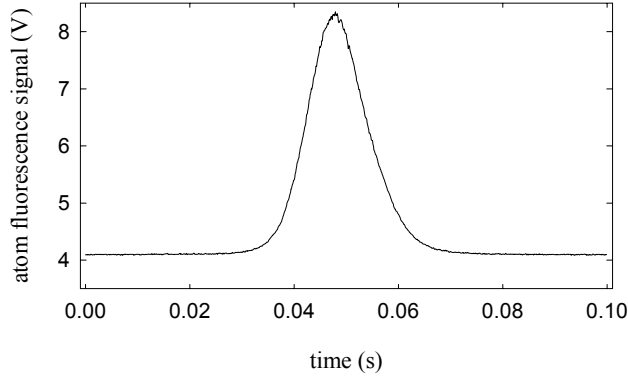
Figure 3. Time-of-flight fluorescence signal for atoms going down through detection region. Area under the curve is proportional to the number of atoms.
