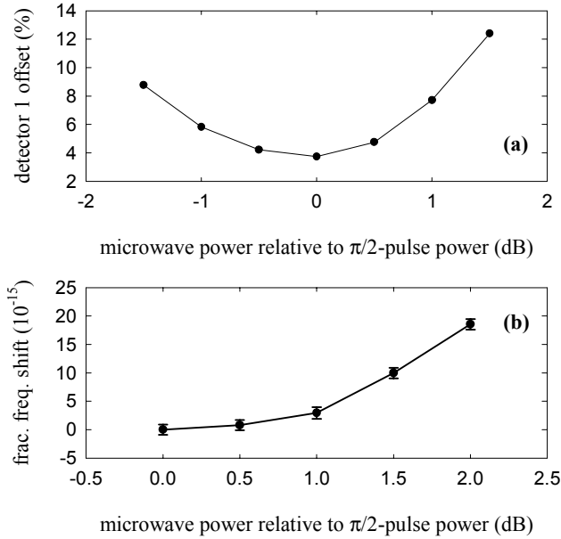
Figure 8. When the microwave power drifts from its ideal value for a \pi/2 -pulse, changes occur to the detector offsets and to the measured clock frequency. Detector 1 offsets (a) and fractional frequency shifts (b) are shown as a function of applied microwave power. Detector 1 offset measurements are used to monitor the drift in the microwave power, as discussed in the text.
