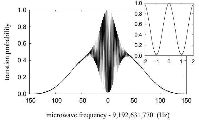
Figure 5. Similar Ramsey fringes to those of Fig. 4, but with each point normalized to the total number of atoms participating in oscillations (i.e. offsets are removed as described in text). Inset shows the normalized central Ramsey fringe with \sim 1 Hz FWHM.
