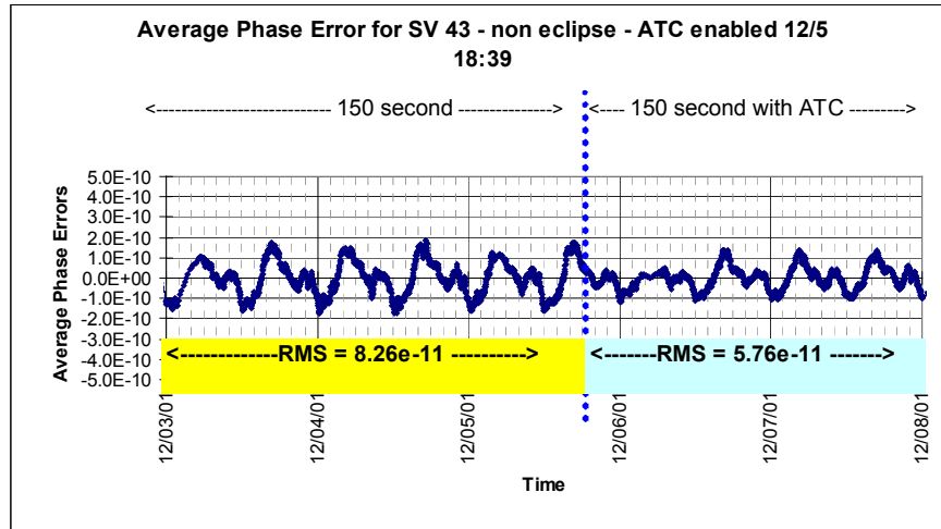
Figure 14. Effect of ATC on orbital phase variation (1/2 hour smoothed data).
