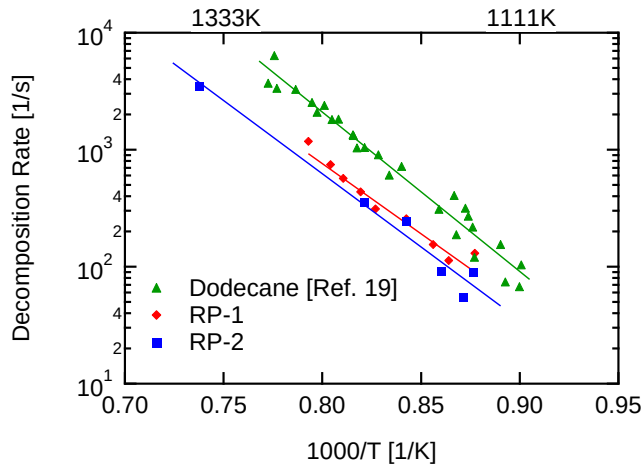
Figure 4. Comparison of decomposition rates for Dodecane, RP-1, and RP-2. Pressure range 3 to 8 atm, 0.2 to 0.5% fuel in argon.
