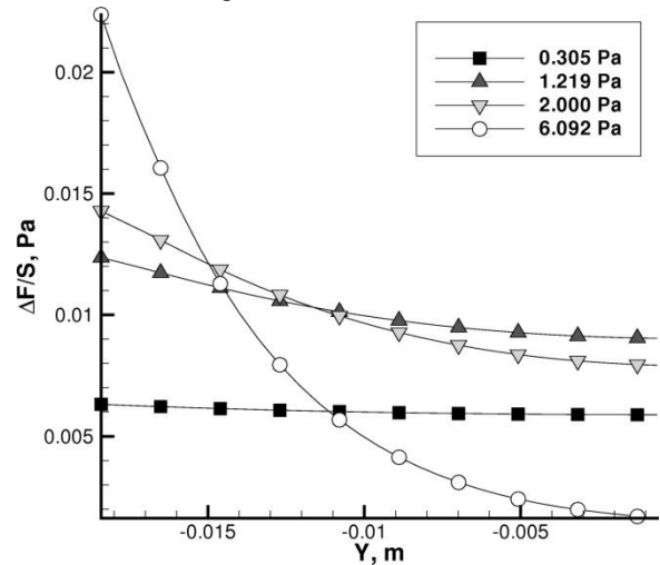
FIGURE 5. Pressure difference along the vane for Ar
