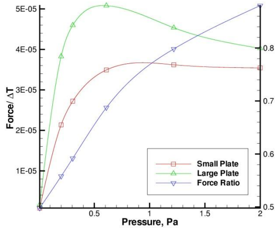
FIGURE 7. Numerical results for two different plates
