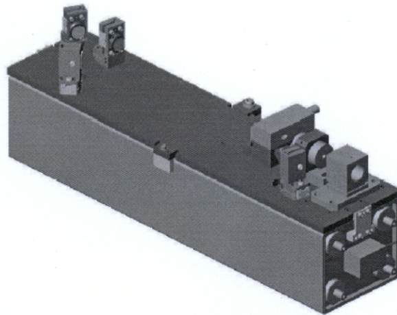
Figure 5: 4430 physics package assembly
