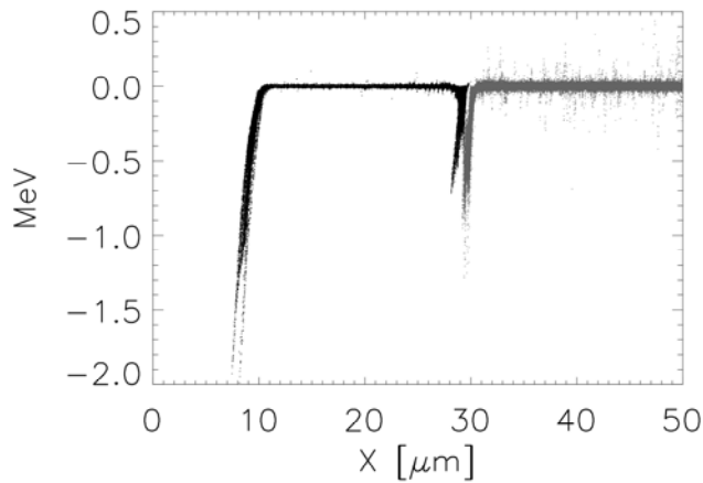
Figure 8: Reverse acceleration of ions in a two material configuration. Laser pulse entered from the left and accelerated the first population. At the interface of the two materials, plasma gets accelerated in backward direction.
