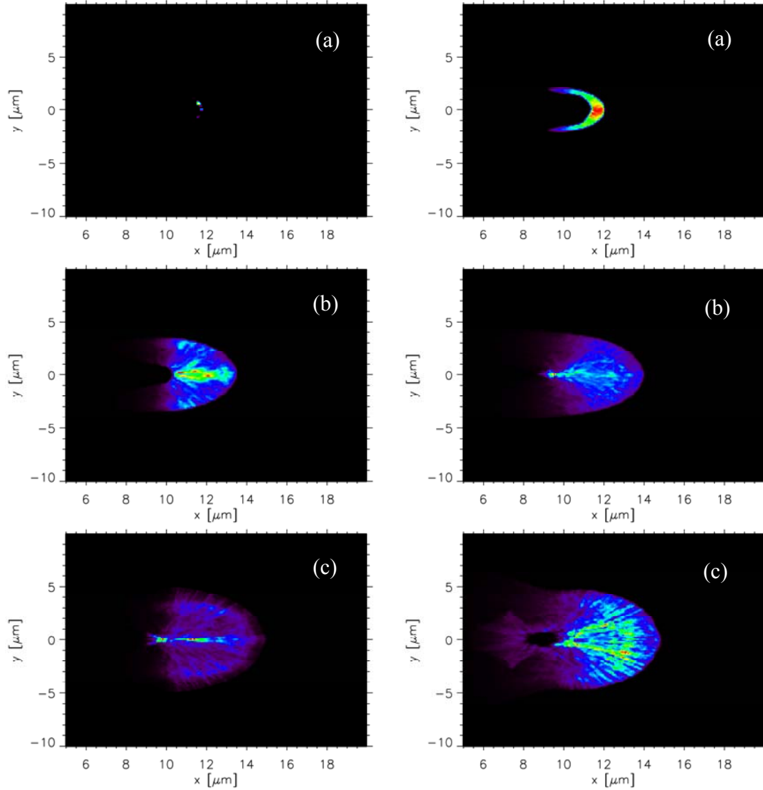
Figure 16: Time evolution of the neutron generation for a laser amplitude of E=3 \times 10^{12} V/m (left) and 6 \times 10^{12} V/m (right) after 0.3ps (a), 0.6ps (b) and 0.9ps (c).
