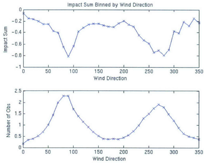
Figure 2: Observed AMV wind direction (degrees) vs. summed observation impact (top panel) and number observations (lower panel)
