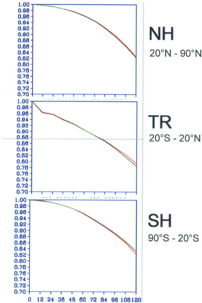
Figure 14: Experiment #2 anomaly correlation of 500 hPa height. Northern Hemisphere (top), tropics (middle), and SH (lower). Control forecasts (red) and EE-threshold forecasts (green). The anomaly correlation differences are not statistically different, although the southern hemisphere forecast skill is slightly improved with the EE-threshold.
