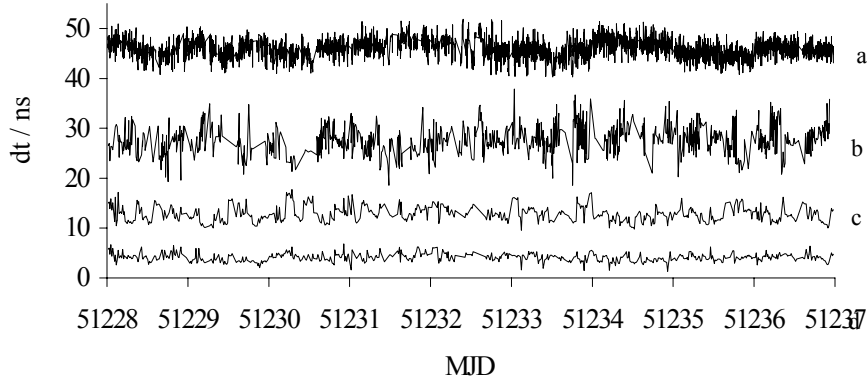
Figure 3. One-site comparisons at the VSL:
