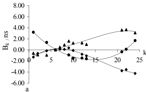
Figure 2. GLONASS P-code frequency biases with respect to frequency No. 6:
