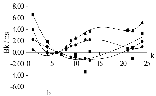
Figure 2. GLONASS P-code frequency biases with respect to frequency No. 6:
