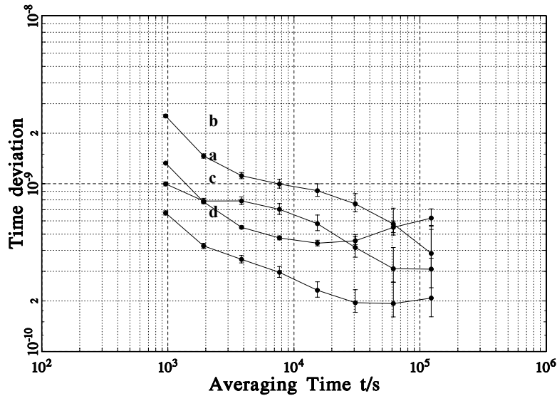
Figure 4. Time deviations for one-site comparisons:
