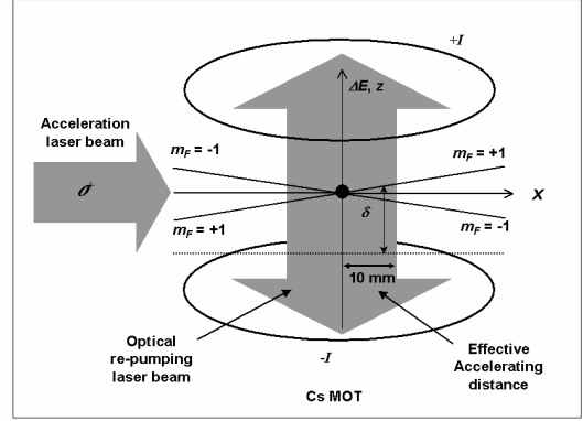
Figure 6. Schematic diagram of the acceleration region of the MOT-based Cs atomic beam. The x-axis is the direction in which the Cs beam travels. The solid, round dot at x = 0, z = 0 represents the trapped Cs atomic cloud. The MOT anti-Helmholtz coils generate an approximately constant magnetic field gradient \partial B / \partial x in the vicinity of the MOT center. The two crossed lines, labeled with m_F = +1 and m_F = -1 , represent the simplified atomic hyperfine levels under Zeeman effects. The vertical axis also stands for the relative energy \Delta E to the atomic resonance, and the horizontal dashed line with \Delta E < 0 indicates the red-detuned acceleration laser frequency. Both the acceleration laser beam and the optical repumping laser beam are circularly polarized. \delta is the total off-resonance detuning of the acceleration laser.
