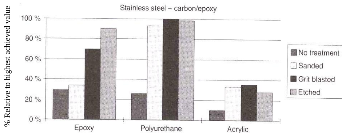
Figure 36: Steel-carbon/epoxy single-lap joint surface treatments and adhesives [30].
