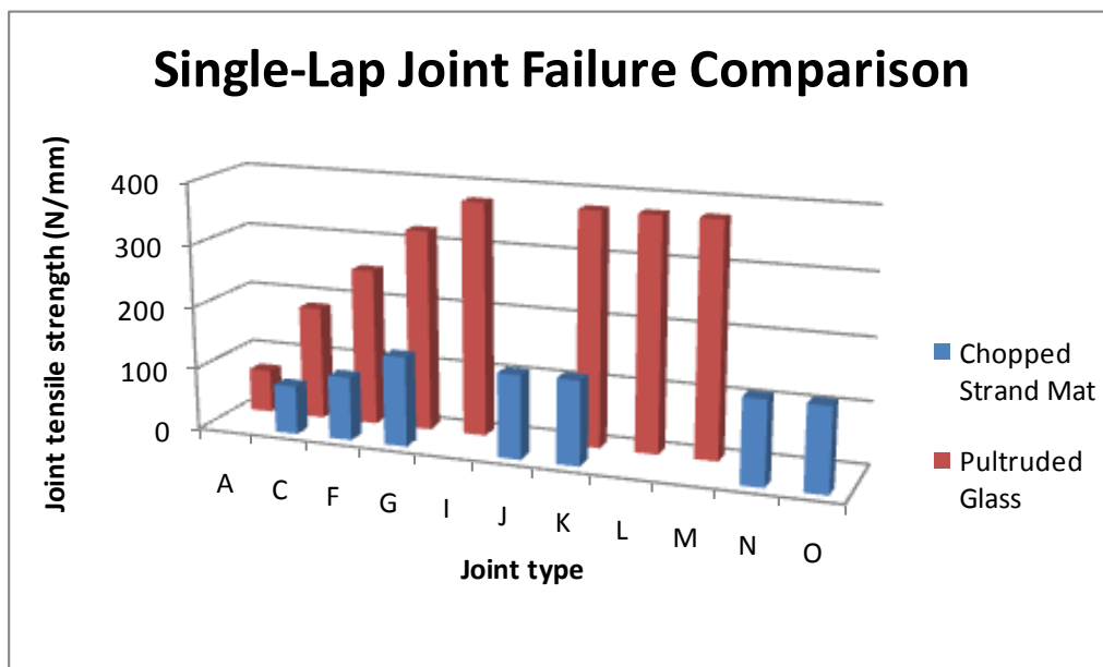
Figure 22: Single-lap joint failure comparison [30].
