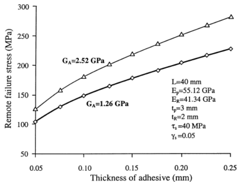
Figure 26: Failure stress versus adhesive thickness [60].
