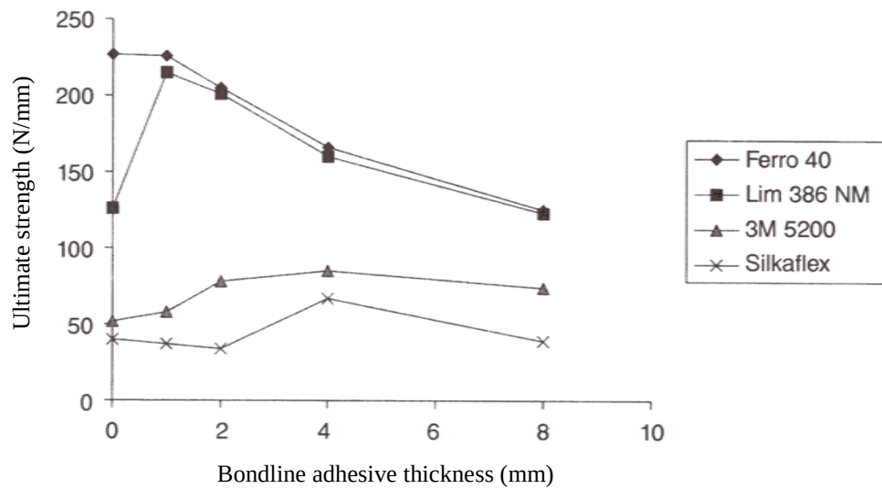
Figure 30: Single-lap joint bondline thickness versus ultimate strength [30].
