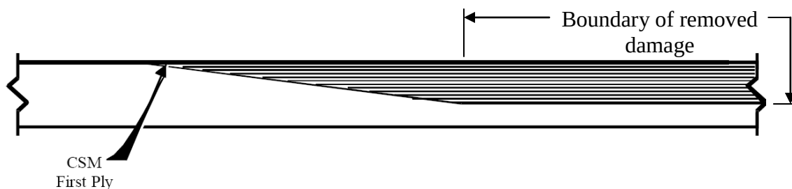
Figure 43: Shortest ply first method [73].
