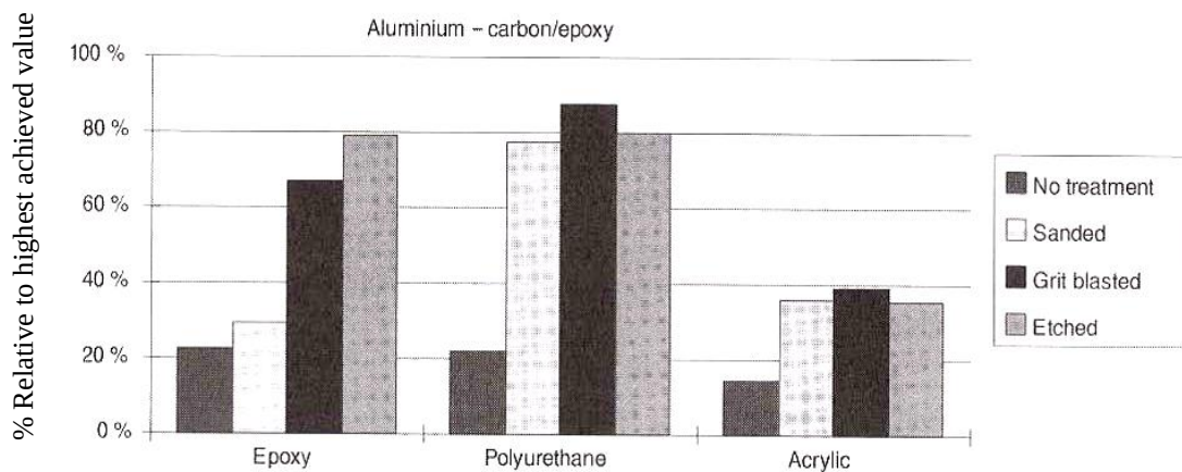
Figure 34: Aluminum-carbon/epoxy surface treatments and adhesives [30].
