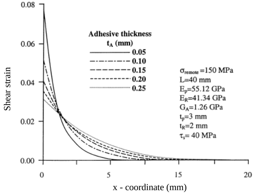
Figure 28: Patch end shear strain versus adhesive thickness [60].
