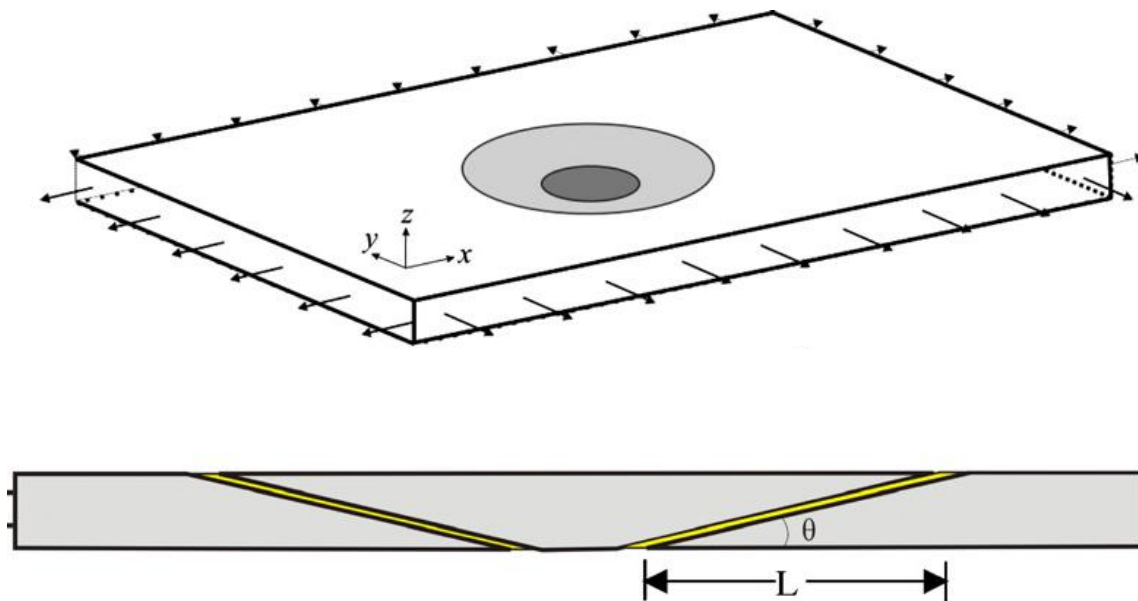
Figure 19: Scarf repair angle [49].
