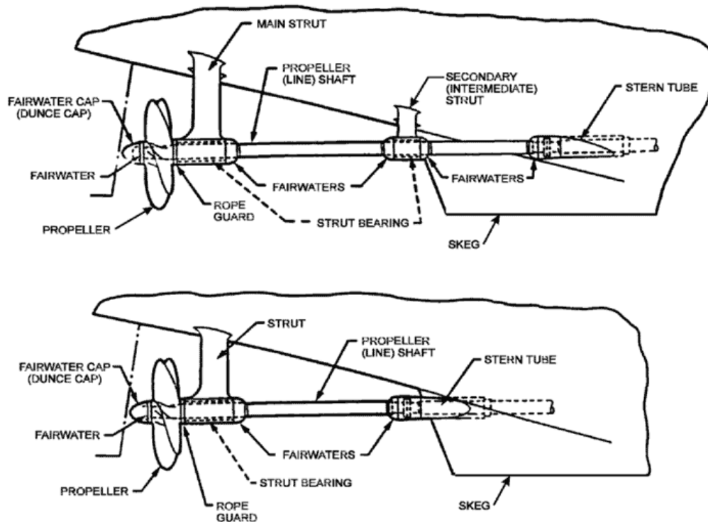
Figure 38: Typical shafting arrangements for U.S. Navy ships [5].
