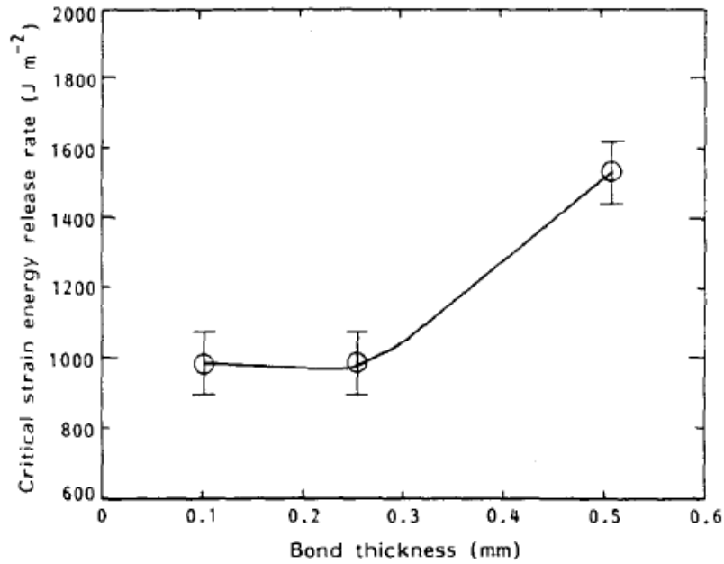
Figure 27: Critical failure energy versus thickness [61].
