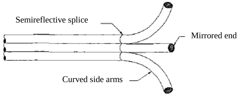
Figure 47: Fabry-Perot rosette sensor [19].
