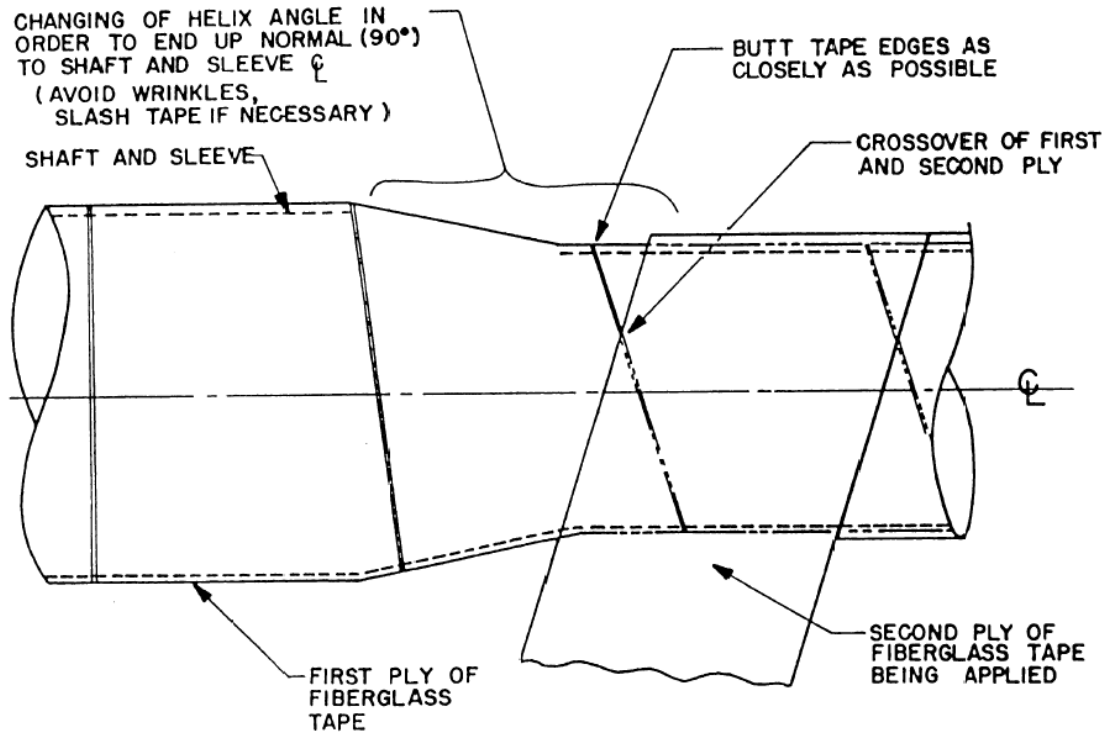
Figure 40: Schematic of FRP wrap [72].
