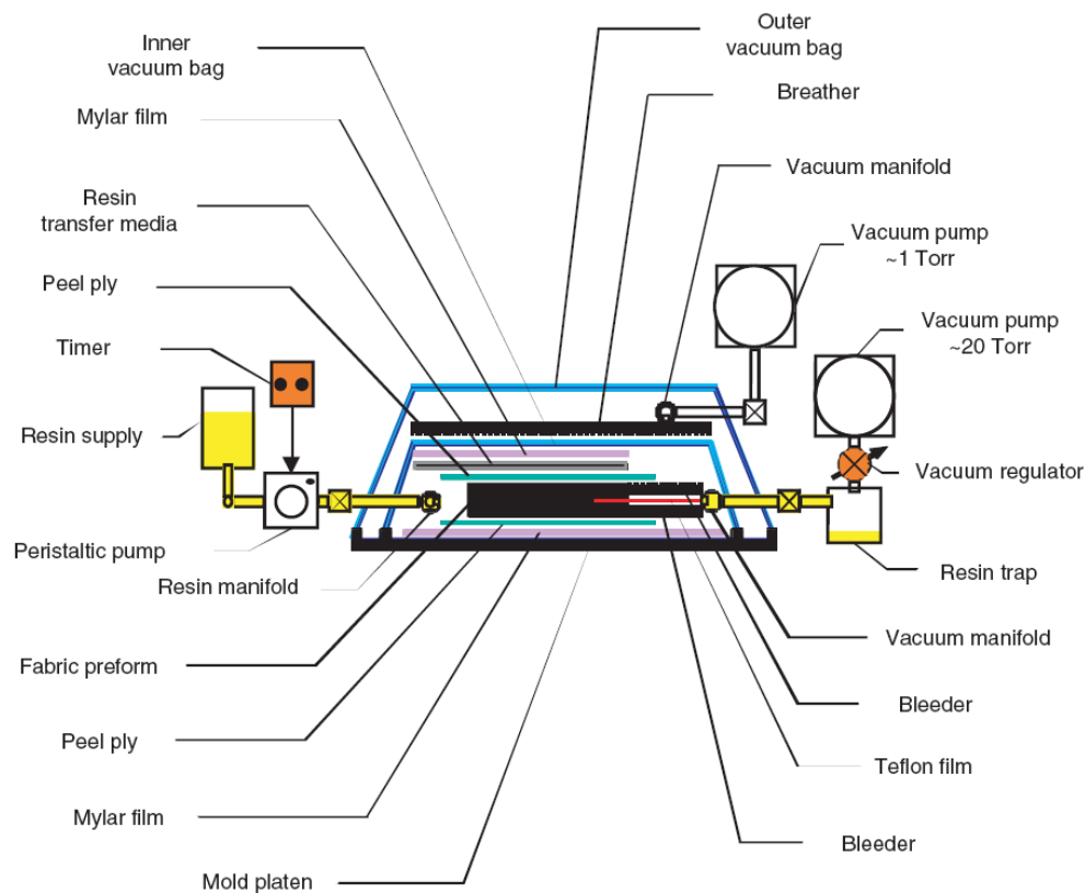
Figure 37: Vacuum assisted resin transfer molding (VARTM) configuration [65].
