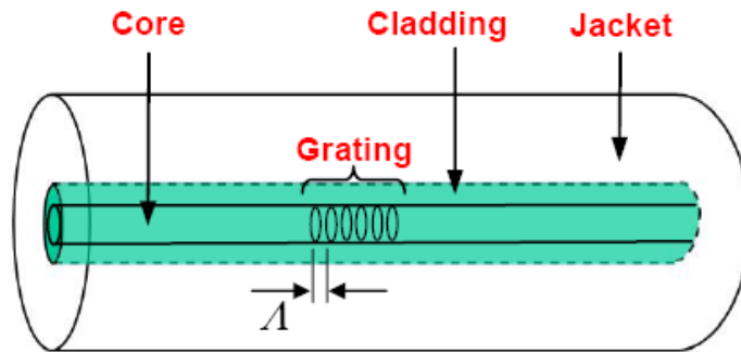
Figure 46: Fiber Bragg Grating (FBG) sensor [81].
