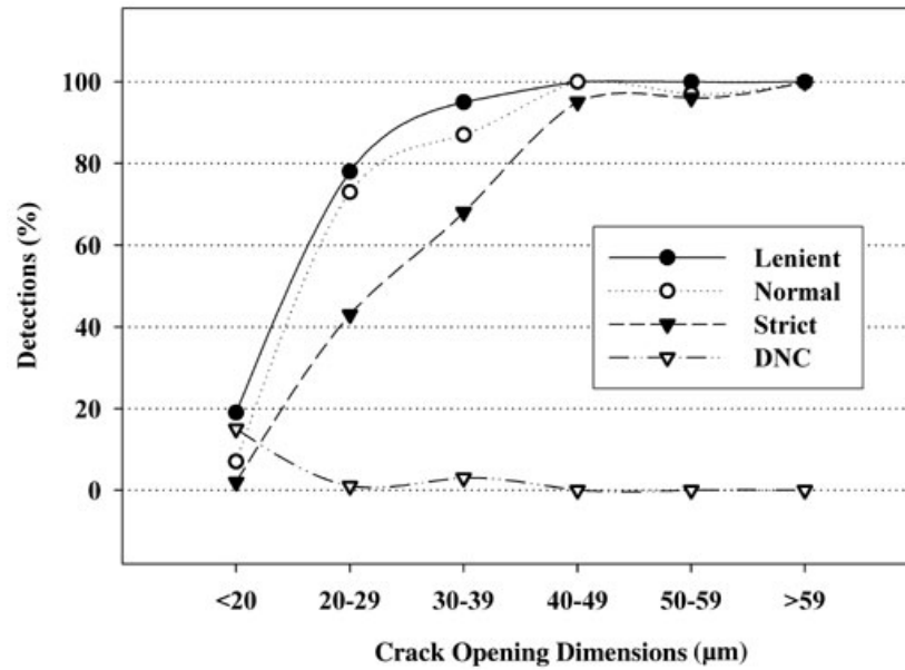
Figure 1: Crack width versus detection underwater [38].
