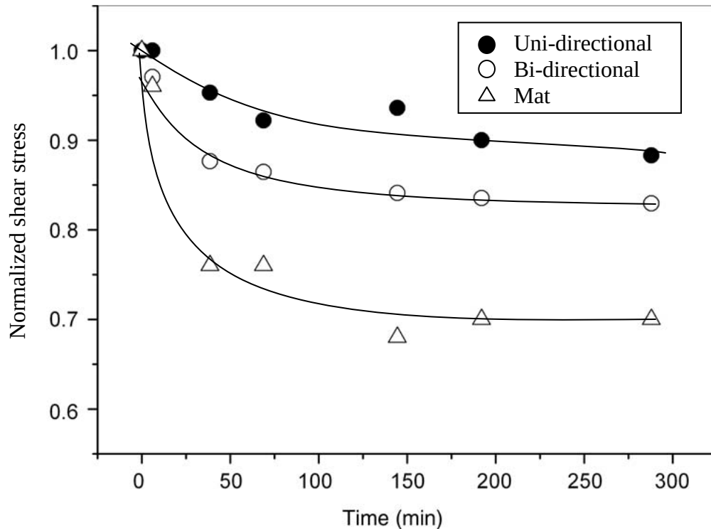
Figure 13: Resistance to shear stress during water immersion at 80°C [46].
