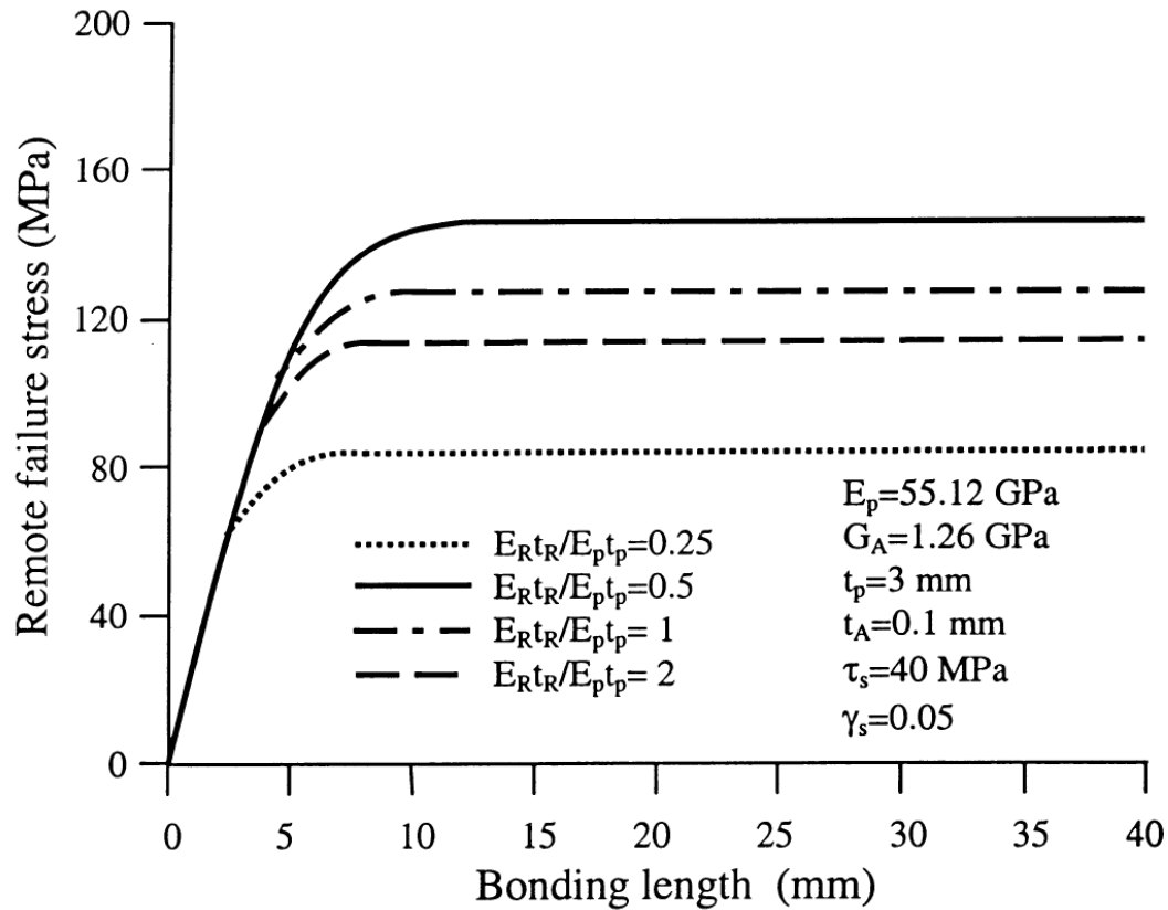
Figure 31: Failure stress of double-lap joint versus bond length [60].
