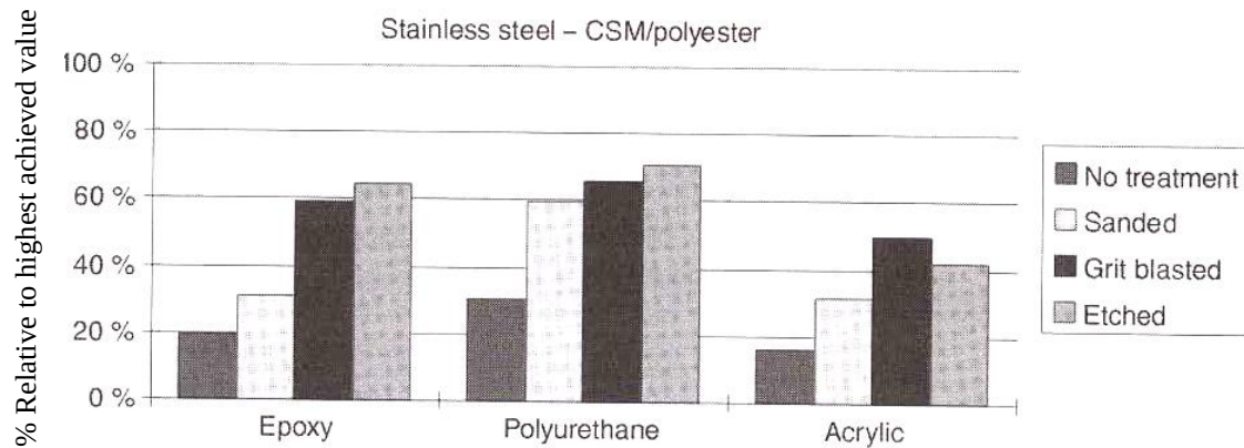
Figure 35: Steel -CSM/polyester single-lap joint surface treatments and adhesives [30].
