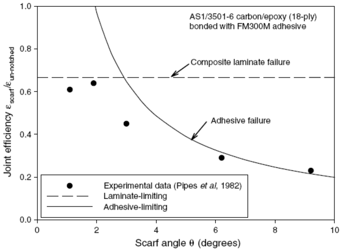
Figure 21: Optimized scarf angle: experimental & predicted [49].
