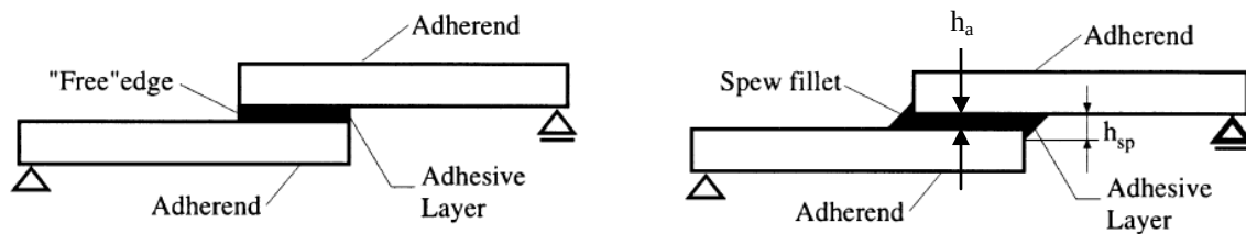
Figure 23: Adhesive bond without and with spew fillet [58].
