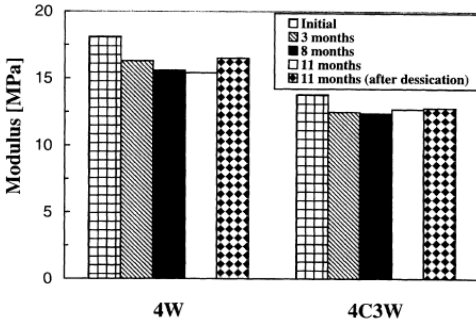
Figure 11: Retention of flexural modulus after immersion in salt solution [50].
