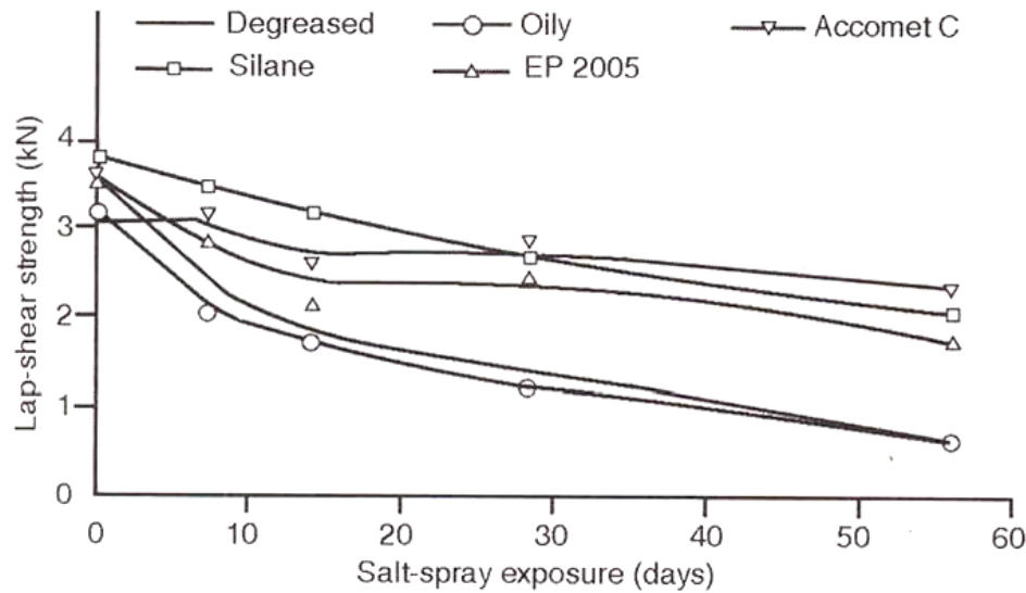
Figure 32: Effect of salt spray correlated to preparation methods [30].
