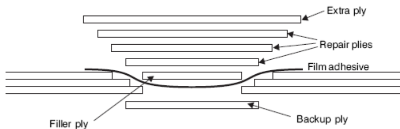
Figure 18: Step sanded repair [62].
