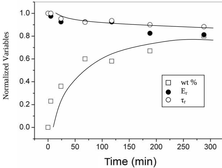
Figure 9: Water absorption for mat composite, glass fiber / vinyl ester [46].
