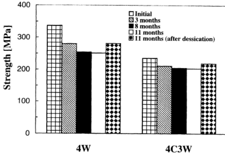
Figure 10: Retention of strength after immersion in salt solution [50].
