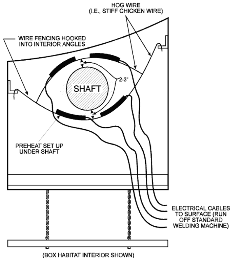
Figure 39: Underwater habitat configuration [5].
