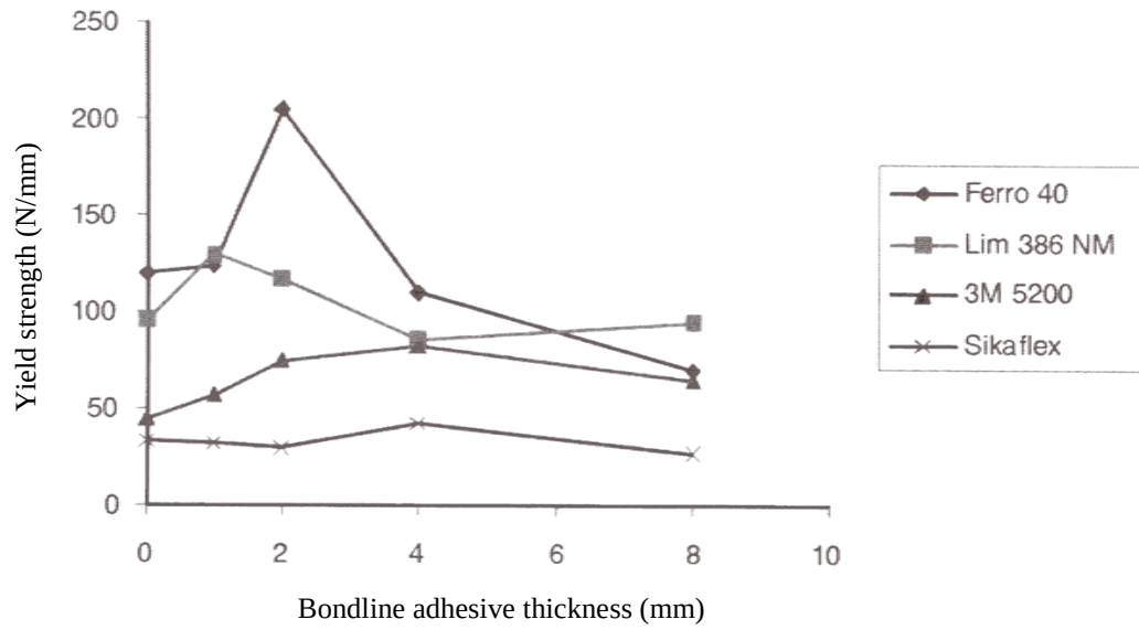
Figure 29: Single-lap joint bondline thickness versus strength [30].
