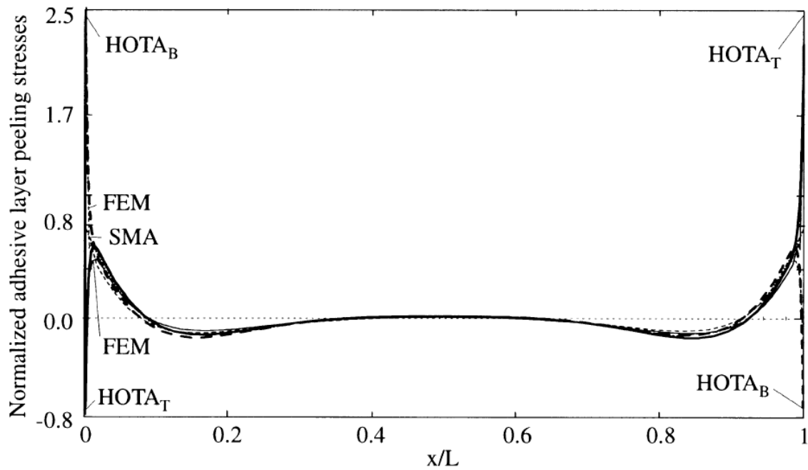
Figure 25: Bondline peel stress without fillet for joint of length (L) [58].
