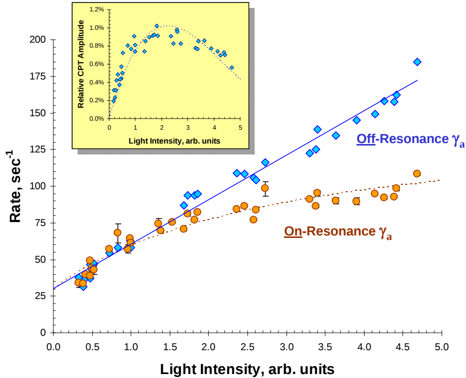
Figure 3. The “slow” decay rate, \gamma_a , for the cases of the sidebands tuned off-resonance and on-resonance as a function of relative light intensity. The inset shows the amplitude of the CPT signal as a function of relative light intensity. The dashed line is simply an aid to guide the eye.
