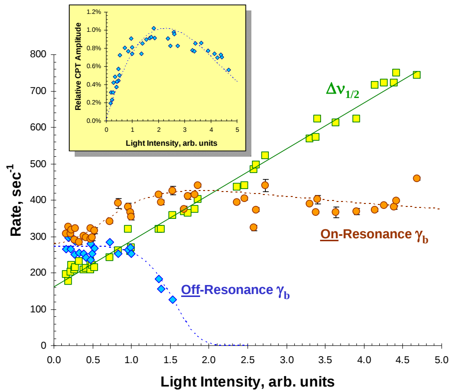
Figure 4. The “fast” decay rate, \gamma_b , for the cases of the sidebands tuned off-resonance and on-resonance as a function of relative light intensity. The inset shows the amplitude of the CPT signal as a function of relative light intensity. The dashed lines are simply aids to guide the eye.
