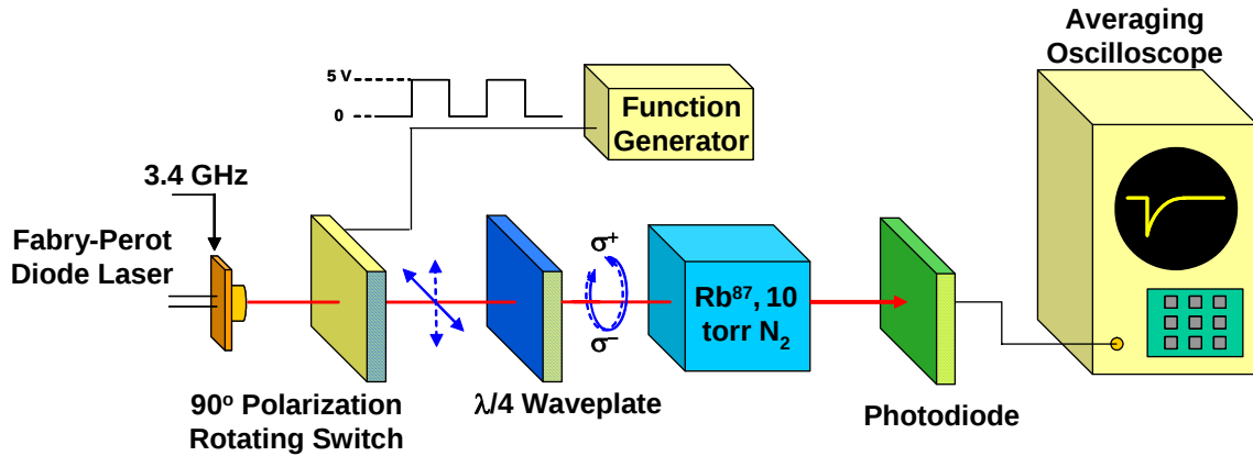
Figure 2. Experimental arrangement. Though not shown, we phase-modulate the field at 3.4 GHz by passing the diode laser output through an electro-optic modulator. The resonance cell contains 10 torr of N_2 as a buffer gas, and sits in a static magnetic field of 0.9 G supplied by Helmholtz coils. The cylindrical resonance cell is 3.9 cm long and is maintained at 46°C.
