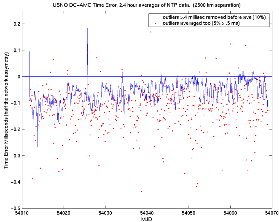
Figure 4. Observed error in NTP Time transfer between USNO-DC and USNO-AMC. Blue plot shows 0.1-day averages when the 10% of the data exceeding 0.4 ms error are removed. Red dots are simple 0.1-day averages of all the data, of which 5% exceed 0.5 ms deviation.
