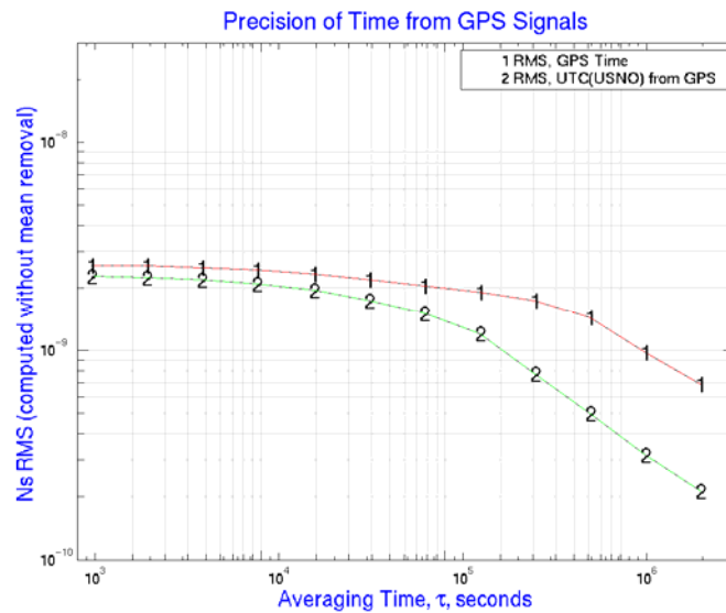
Figure 6. The precision of GPS Time and of GPS's delivered prediction of UTC (USNO), using TTR-12 data since 7 February 2005, measured by the attainable external precision (rms, mean not removed) as a function of averaging time, and referenced to UTC (USNO). Improved performance in accessing UTC (USNO) could be realized if only the most recently updated navigation messages are used. The accuracy attainable over a given averaging time also depends upon the calibration of the user's receivers.
