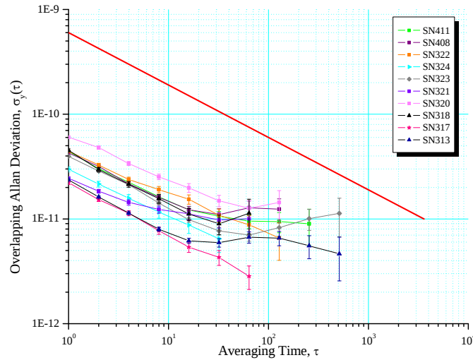
Figure 11. Short-term frequency stability of 10 Phase-III physics packages. CSAC performance objective of \sigma_y(\tau=1) < 6 \times 10^{-10} is shown in red.
