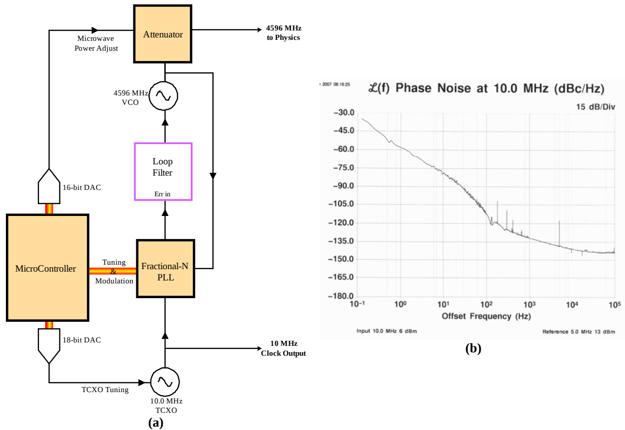
Figure 12. (a) Block diagram of the CSAC microwave synthesizer and (b) SSB phase noise of 10.0 MHz output.
