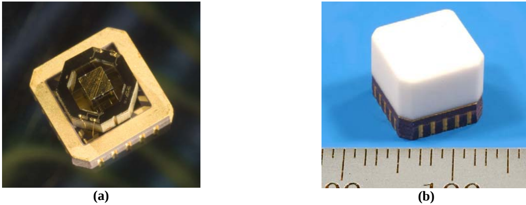
Figure 5. (a) Phase-III physics package in LCC and (b) sealed Phase-II physics package (Phase-III is similar).
