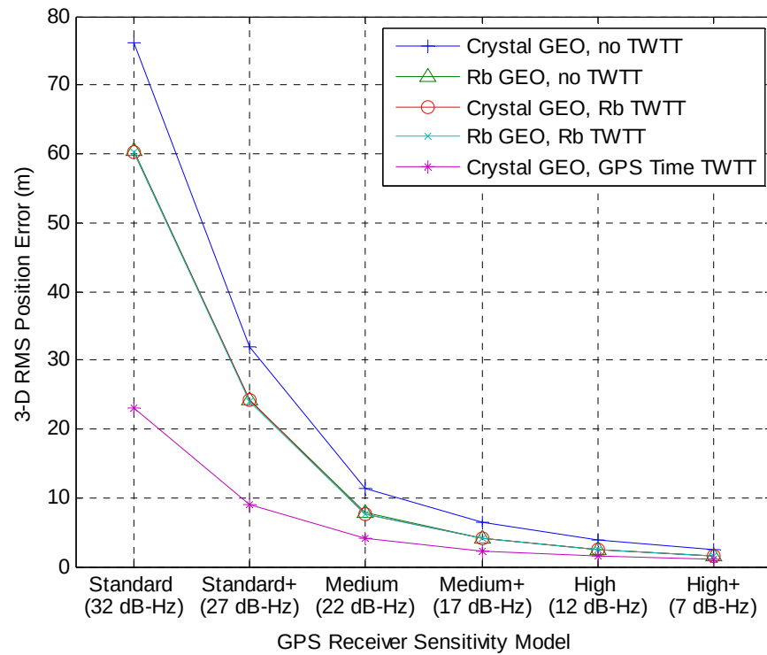
Figure 9. 3D RMS position error vs. GPS receiver sensitivity levels for five basic scenarios.
