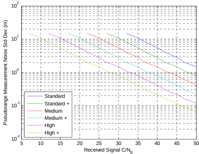
Figure 6. Simulated receiver models.
