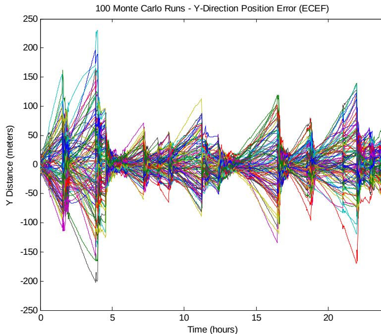
Figure 7. 100 Monte Carlo runs, standard receiver, ovenized crystal oscillator, no TWTT measurements.
