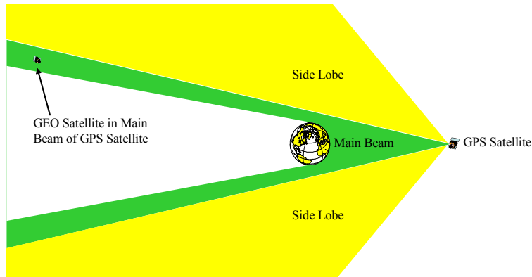
Figure 1. GPS/GEO satellite coverage geometry.
