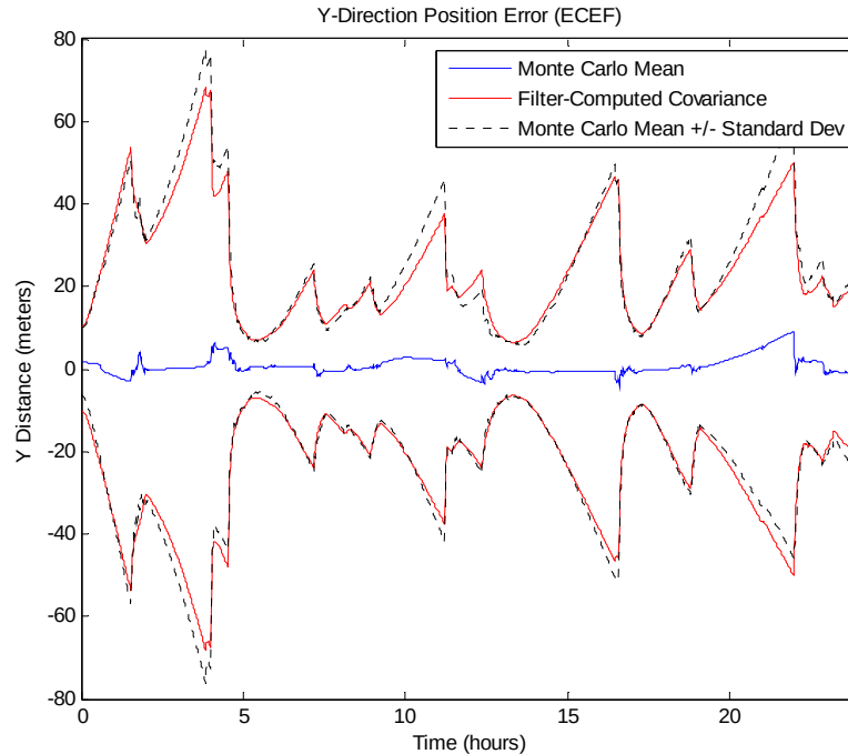
Figure 8. Comparison between Monte Carlo ensemble statistics and filter-computed statistics, standard receiver, ovenized crystal oscillator, no TWTT measurements.
