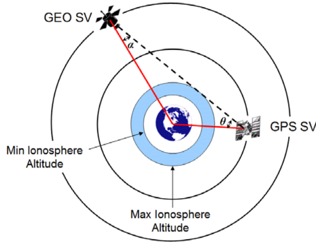
Figure 5. GPS measurement geometry.
