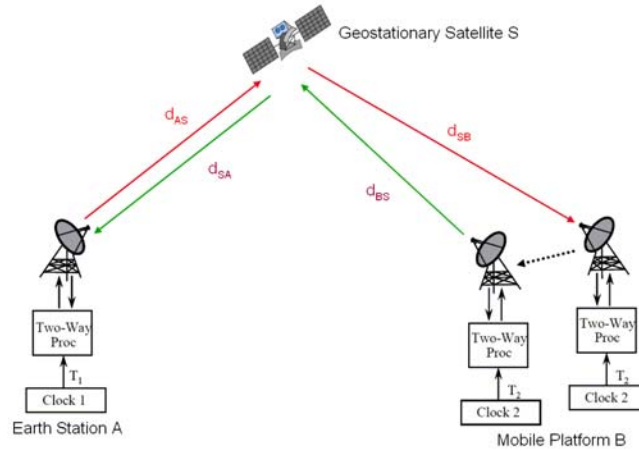
Figure 3. Dynamic TWTT using a satellite [2].
