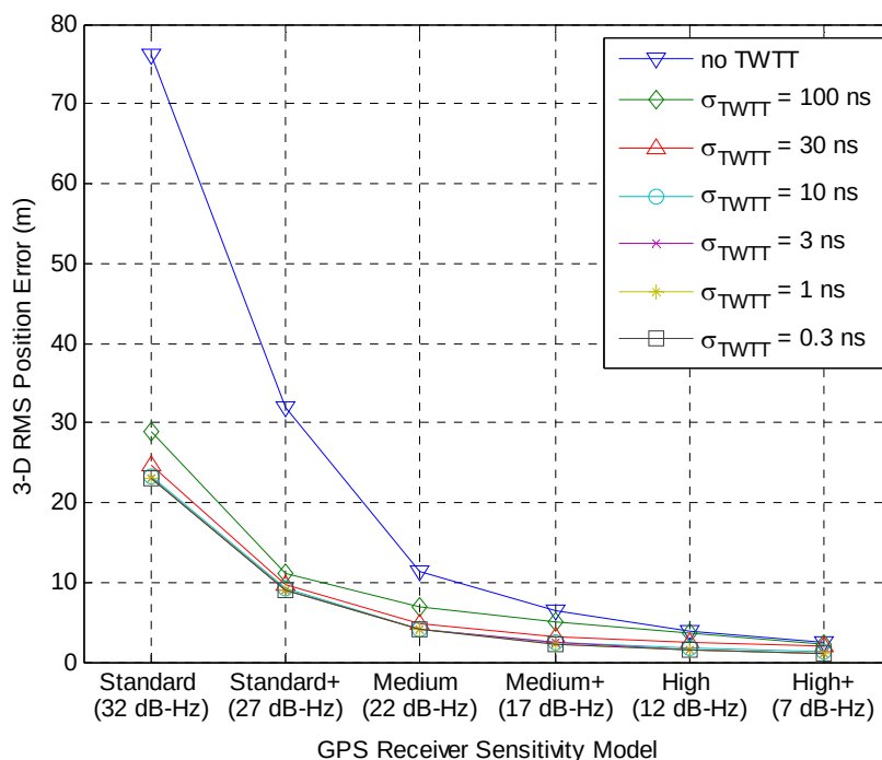
Figure 11. 3-D RMS position error for varying TWTT measurement errors for Scenario 5 (TWTT with reference clock synchronized with GPS Time).
