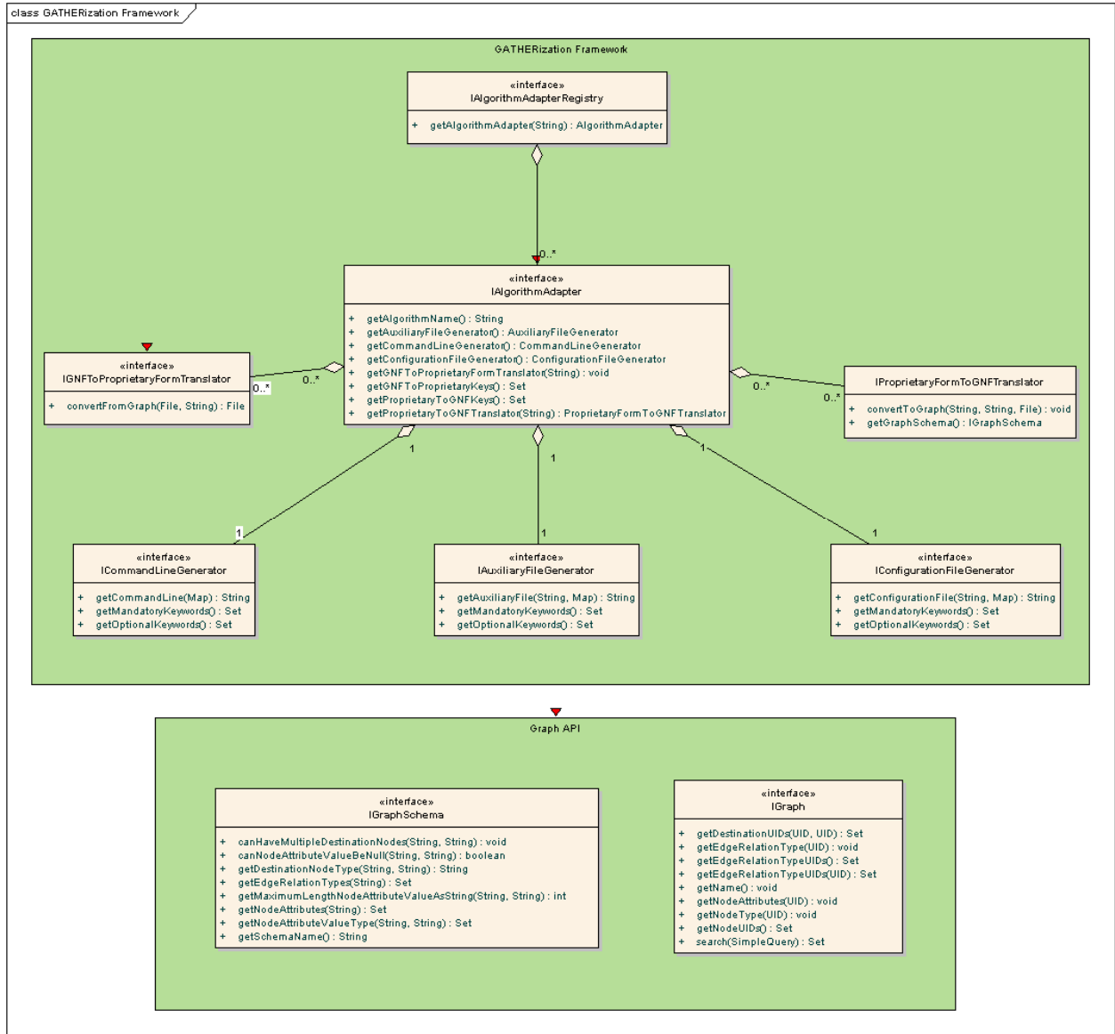
Figure 6: GATHER Framework
