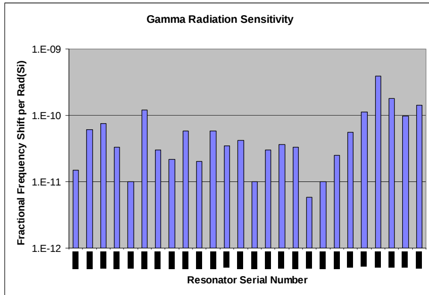
Figure 9. Fractional frequency shift in BG-61 resonators per rad (Si), gamma.
