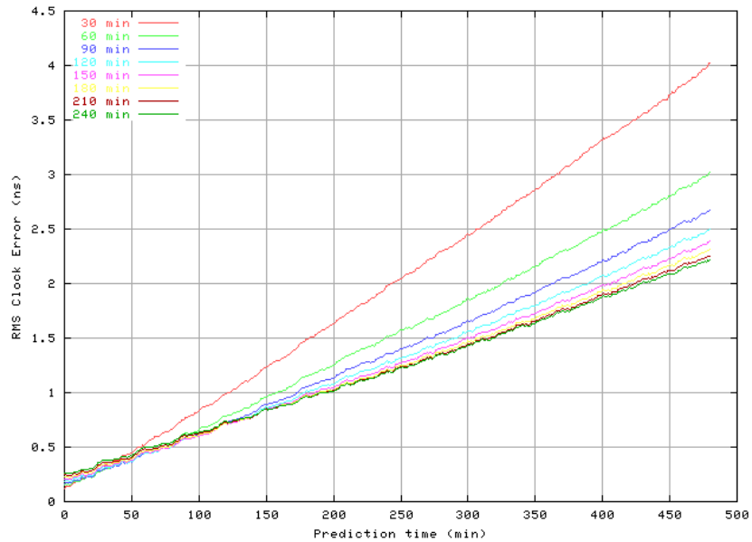
Figure 1. Block IIR clock predictability analysis (linear fit – PRN: 11, 13, 20, 28).
