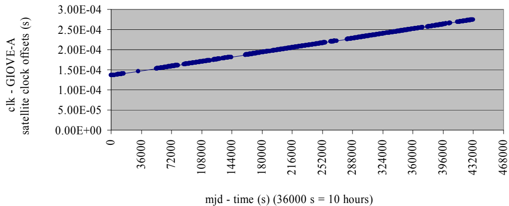
Figure 6. GIOVE-A satellite clock estimation ( af_2 = 5.19 \cdot 10^{-18} s/s 2 ).
