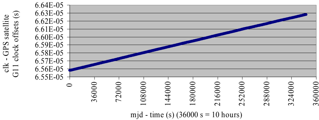
Figure 5. Satellite G11 clock estimation ( af_2 = -1.37 \cdot 10^{-19} s/s 2 ).
