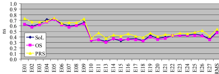
Figure 11. Clock estimation accuracy (RMS over a 6-hour estimation period).
