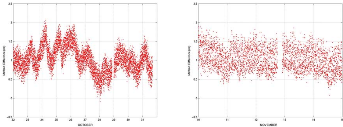
Figure 12. The graphs above shows the difference between GPS link and fiber link. The left graph shows periodic variations in October before change of H-maser and other equipment at STUPI. The right graph shows the difference between the systems after changes; the oscillations are gone, but the noise has been increased.
