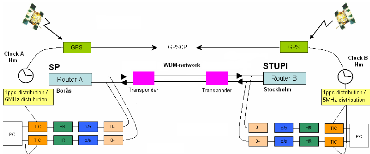
Figure 6. The setup for the 500-km baseline experiment of a fiber time transfer link with GPS carrier-phase link for comparison and evaluation.
