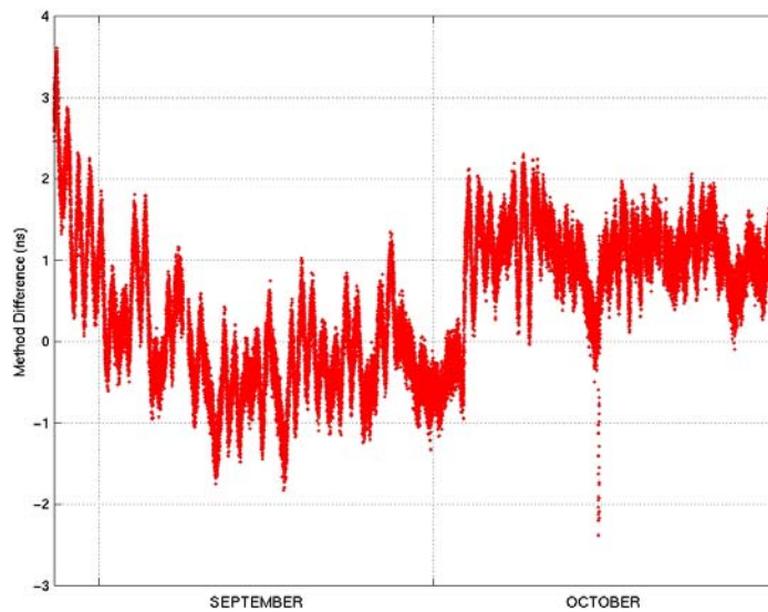
Figure 11. Difference between GPS link and fiber link during time period 3 (see text). The rms difference is 860 ps. An arbitrary offset has been removed.
