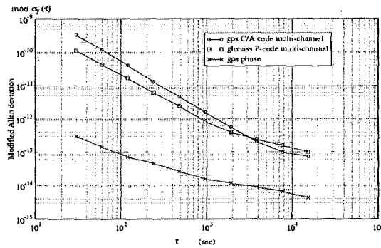
Figure 4: Frequency stabilities of the different time transfer results of Figure 3.
