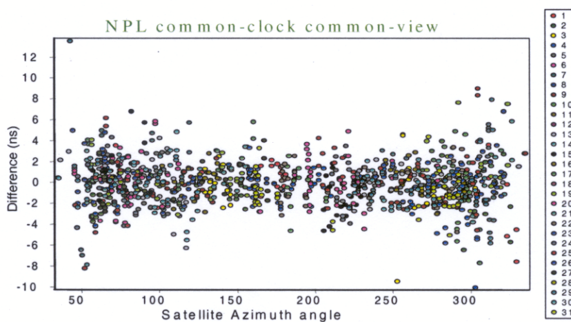
Figure 10 shows the dependence of NPL’s common-clock common-view DFM measurements on satellite azimuth angle.
