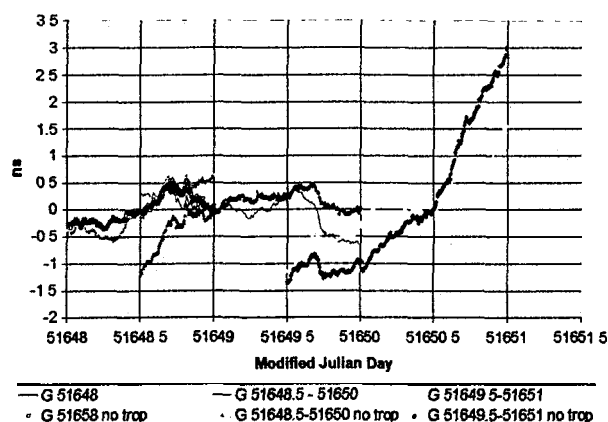
Figure 9: Solutions for runs of 1.5 d with and without troposphere estimation.
