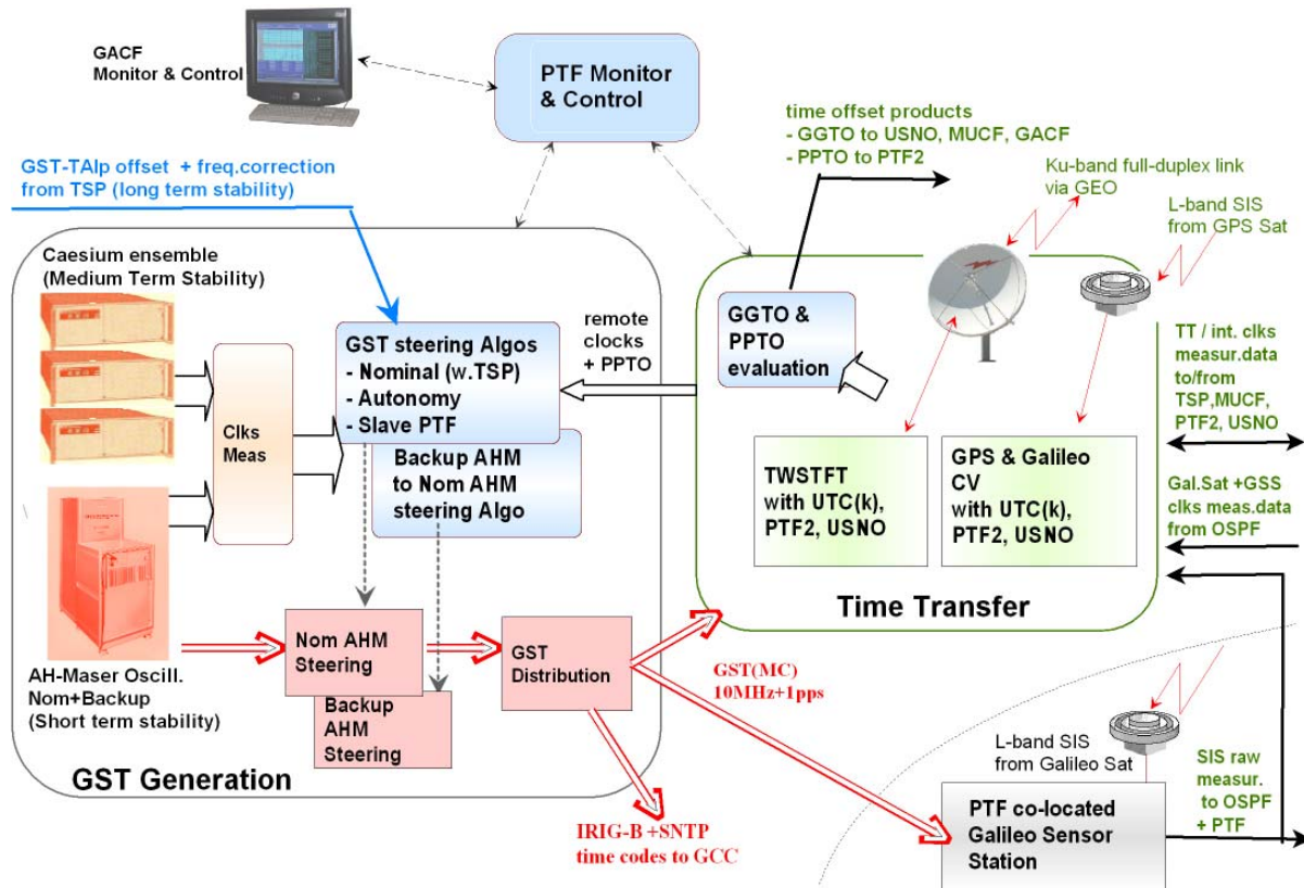
Fig. 3. PTF functional block diagram.
