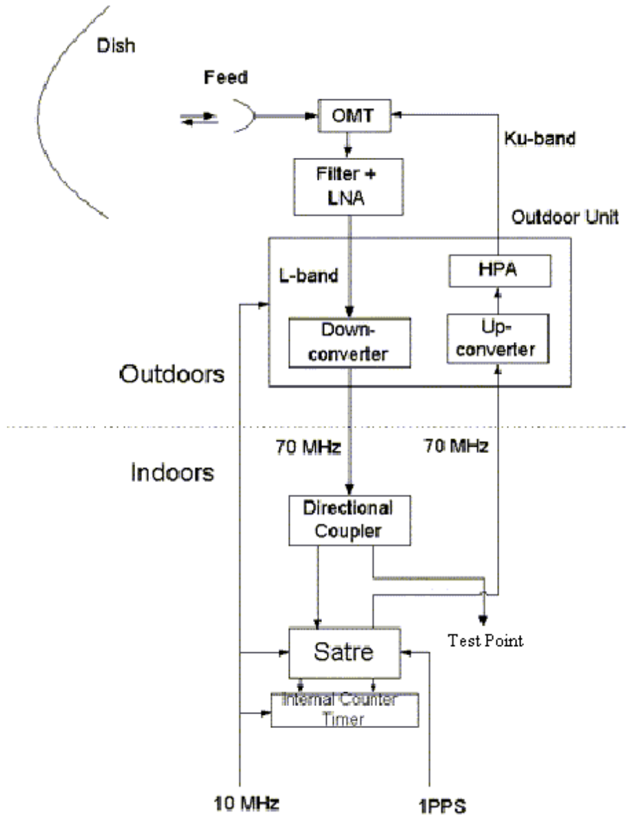
Fig. 4. TWSTFT Station block diagram.
