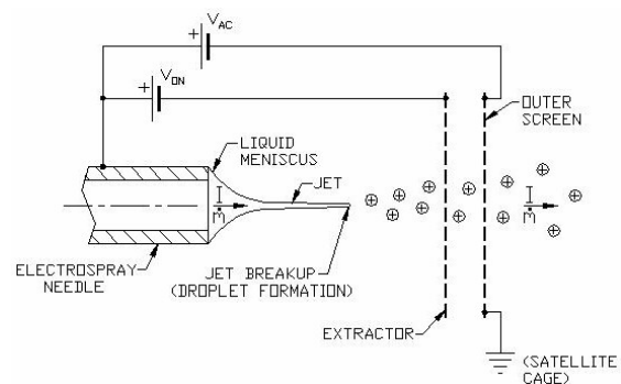
Figure 1: Schematic of Electrospray Thruster
