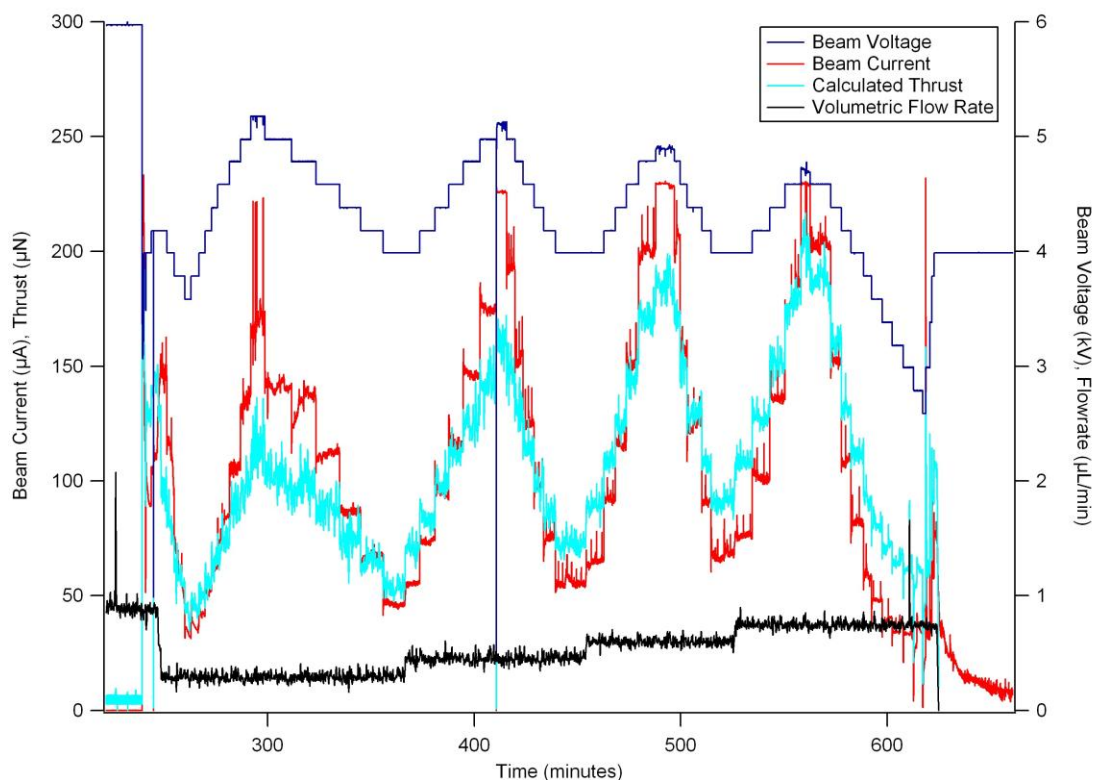
Figure 8: Beam Voltage, Flowrate, and Calculated Thrust from a Run Using a Single Slit Colloid Thruster. Slit emitter is approximately \frac{1}{2} " x \frac{1}{2} " x 2" dimensions.
