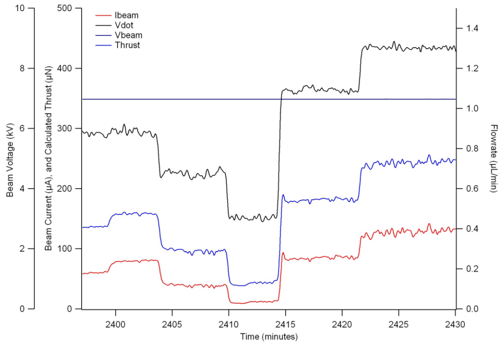
Figure 6: Typical Colloid Thruster Response to Variations in the Delivered Flowrate to the Planar Emitter. The estimated thrust was calculated based on beam current (Ibeam), and voltage (Vbeam) after each test run. The thrust indicated here does not take into account losses associated with plume divergence and droplet voltage loss due to electrospray emission cone formation. Note the thrust levels of 200 \mu N for a single emitter, as opposed to 3-4 \mu N per emitter for the NASA ST7 thrusters.
