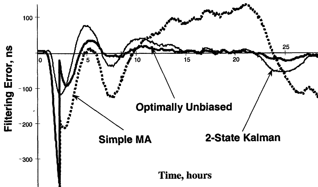
Figure 7. Filtering of the GPS-based time error process generated by the OCXO for \Delta = 100 s, and N = 80 : a) Estimates; b) Errors with respect to the three-state Kalman estimate.
