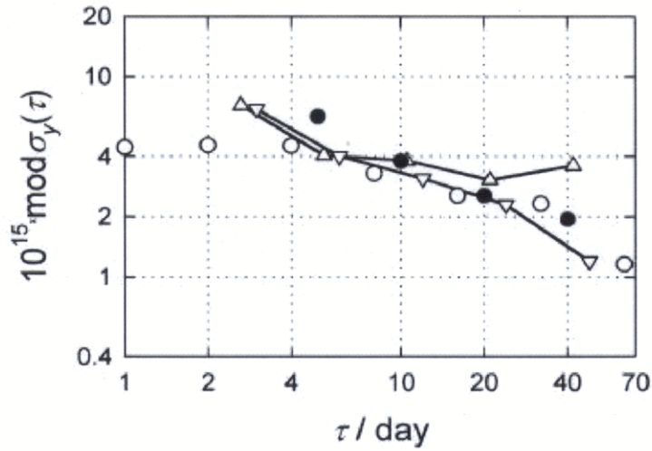
Figure 6. Frequency instability \text{mod } \sigma_y(\tau) observed in the comparison between TAF(PTB) and TAI (●), TAF(PTB) and UTC(USNO) using TWSTFT (△), TAF(PTB) and UTC(NIST) using TWSTFT (△), TAF(PTB) and NIST AT1E (O) using GPS carrier-phase results provided by L. Nelson, USNO (previously NIST). TWSTFT data were rearranged as if they were taken at regular intervals.
