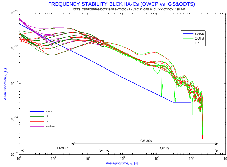
Figure 2. Block II-A Cs clocks, ADEV for 2007 doy 138-142.
