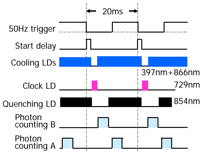
Figure 6. The timetable for the pulse-light sequence. The “counting A” detects that the ion is in the cooling cycle. The “counting B” checks the counting rate to determine if the quadrupole transition occurred. The “50 Hz trigger” synchronizes with east Japan’s main electricity.
