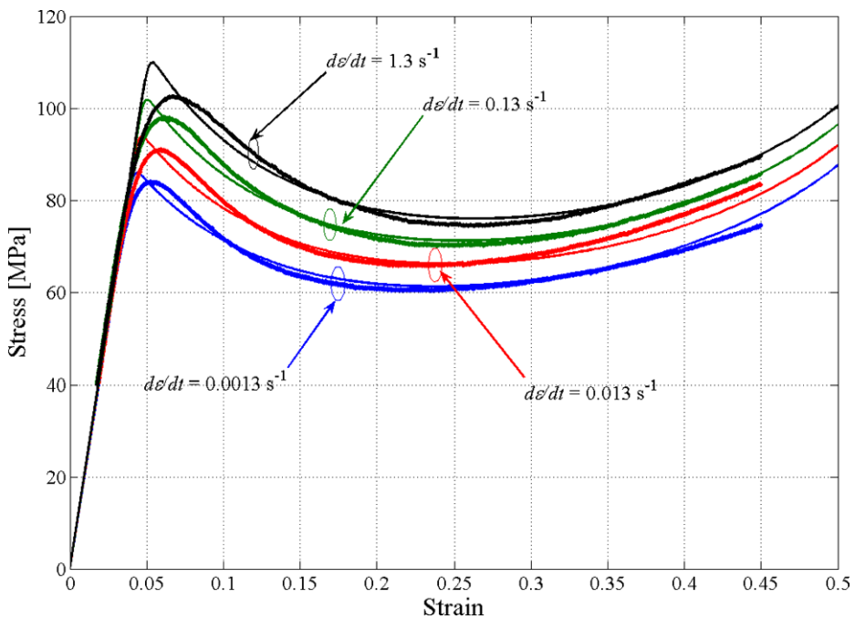
Fig. 11 The stress-strain relationship predicted from the 1-D Mulliken-Boyce model ( solid line ) using the parameter estimates in Table 3 for low strain rate. The experimental data ( heavy dotted line ) is plotted, showing the excellent agreement
