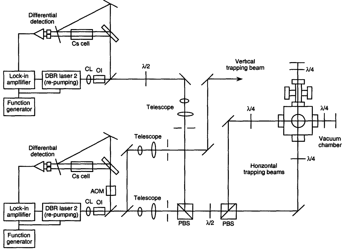
Figure 2. Simplified schematic diagram of the Cs magneto-optical trap testbed. The vacuum chamber has a background pressure < 1 \times 10^{-9} Torr and contains Cs atomic vapor at a controlled pressure. Two frequency-stabilized diode lasers provide the cooling/trapping and optical re-pumping beams. AOM: acousto-optical modulator, CL: collimation lens, OI: optical isolator, PBS: polarization beam splitter, \lambda/2 : half-wave waveplate and \lambda/4 : quarter-wave waveplate. A third diode laser (not pictured) is used to provide laser-induced fluorescence for the time-of-flight measurements of the cold atomic beam.
