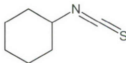
Figure 1. Structure of Cyclohexyl Isothiocyanate
