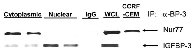
Fig. 1. Cytoplasmic interaction between IGFBP-3 and Nur77. 22RV1 cells were taken serum free overnight and association of endogenous Nur77 and IGFBP-3 was assessed. Nuclear and cytoplasmic fractions were isolated as indicated. Protein A-agarose was used to immunoprecipitate bound complexes and resolved by SDS–PAGE. Nur77 and IGFBP-3 were detected by immunoblotting. 22RV1 whole-cell lysate (WCL) was used as an input control. CCRF-CEM nuclear extract as a positive control for Nur77 presence. Experiments were repeated three times.
