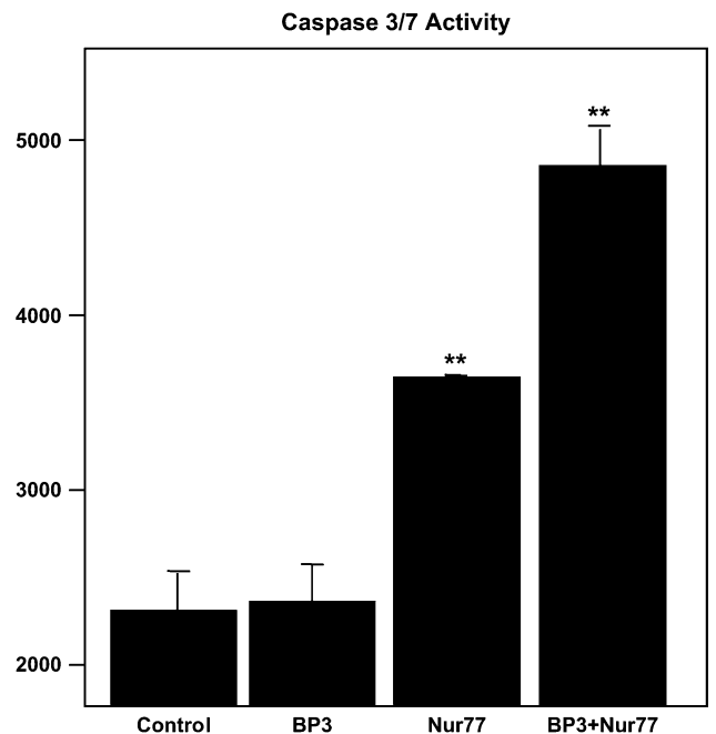
Fig. 3. Reintroduction of Nur77 into Nur77 KO MEFs restores responsiveness to IGFBP-3. Values are normalized to \beta -galactosidase expression to adjust for transfection efficiency. ^{**}P < 0.005 relative to control vector alone and also for combination compared with Nur77 alone. Experiments were repeated three times.
