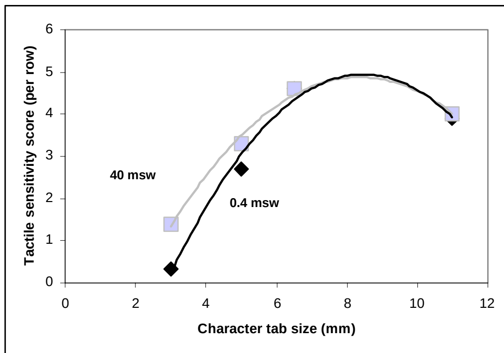
Figure 14: Effect of Tab Size on Tactile Sensitivity Score when wearing Neoprene Gloves in Cold Water
