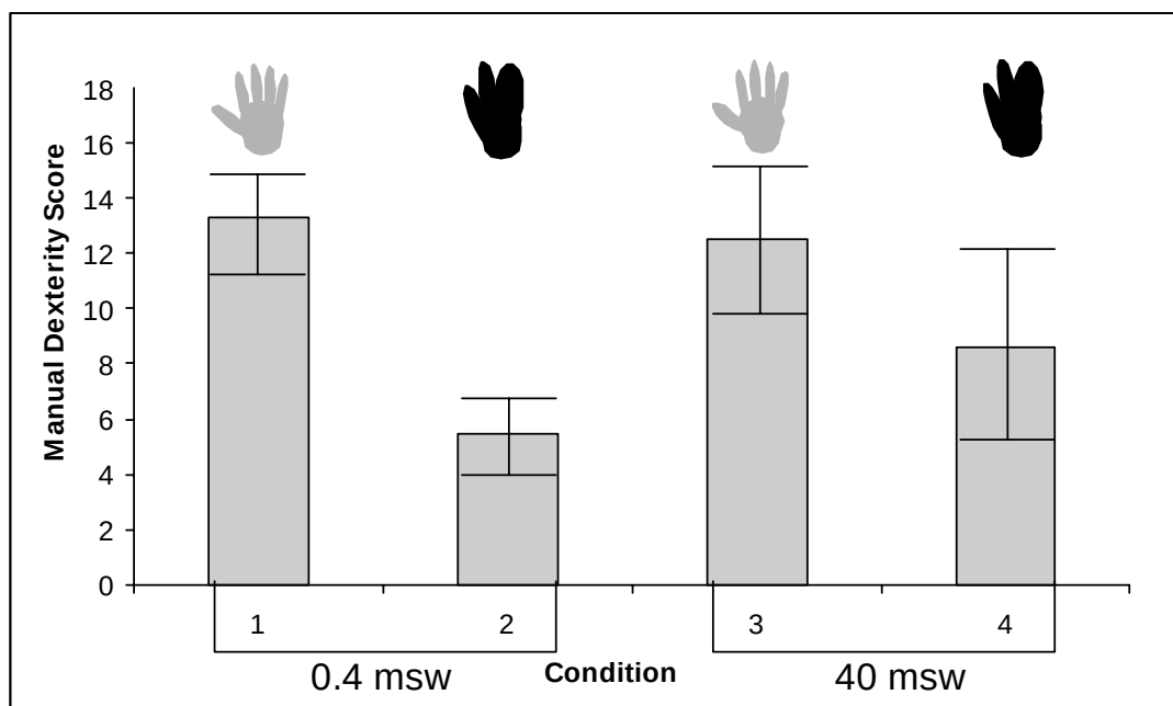
Figure 7: Effects of Pressure and Gloves on Manual Dexterity Score
