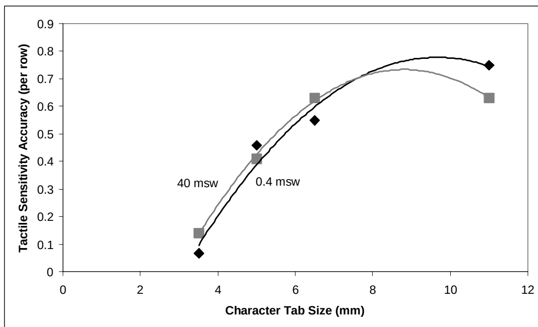
Figure 15: Effect of Tab Size on Accuracy of Tactile Sensitivity when wearing Neoprene Gloves in Cold Water
