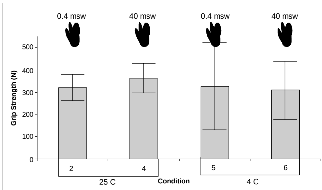
Figure 9: Effects of Temperature and Pressure on Grip Strength
