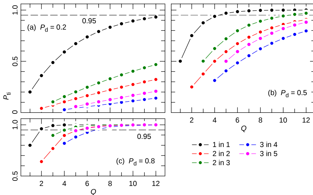
Figure 29: Track-initiation probability for various initiation rules as a function of total number Q of ensonifications considered for P_d = (a) 0.2, (b) 0.5 and (c) 0.8. Each curve starts at the window length of the rule (i.e. at Q = q ). In panel (c), the results for the 3-in-5 rule – starting at Q = 5 – lie essentially on top of those for the 2-in-2 rule. For reference, broken lines mark P_{ti} = 0.95 . Note the suppressed zero in panel (c).
