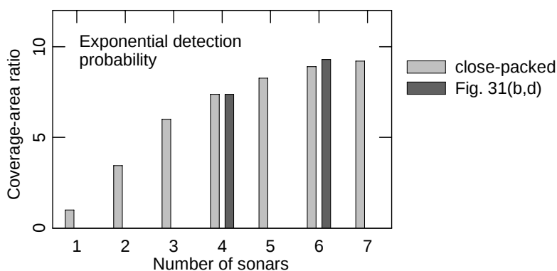
Figure 32: Effect of geometric arrangement on coverage area ratio.
