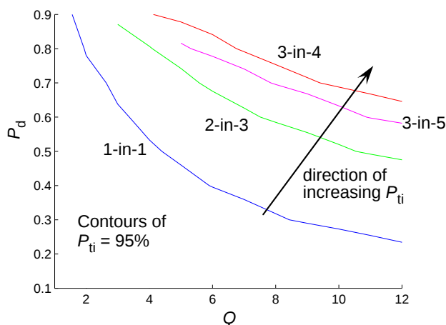
Figure 30: Contours at which P_{ti} = 95\% in the P_d - Q plane for several track-initiation rules. As in Figure 29, each curve starts at Q = q .
