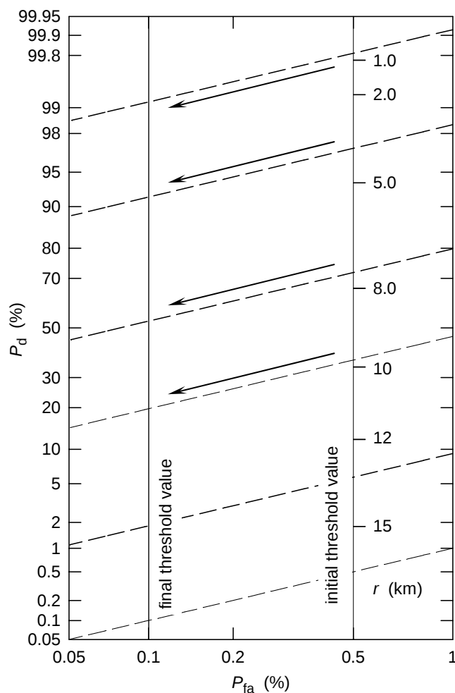
Figure 36: Graphical depiction of the calculation of the effect on P_d of an adjustment in threshold. Both axes use normal-probability coordinates, so that the ROC curves (broken lines) are straight. The two vertical lines represent two threshold values that correspond to false-alarm rates a factor of 5 apart. The scale on the line at P_{fa} = 0.5\% show range values for the Fermi-function P_d behaviour of Figure 3(b). The arrows show how the range values translate with the change in threshold from that with P_{fa} = 0.5\% to that with P_{fa} = 0.1\% .
