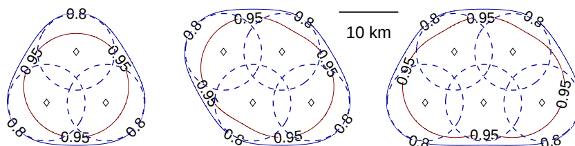
Figure 12: As in Figure 10, but with P_0 = 0.80 . Note the absence of the 95% single-sonar contours (red broken lines in other contour plots).
