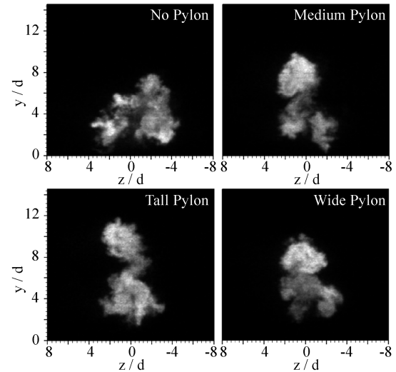
Fig. 5 Instantaneous NO-PLIF end-view images ( x/d = 16 ).
