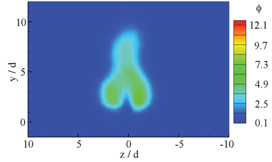
Fig. 13 Equivalence-ratio contours for case 9 ( x/d = 12 ).
