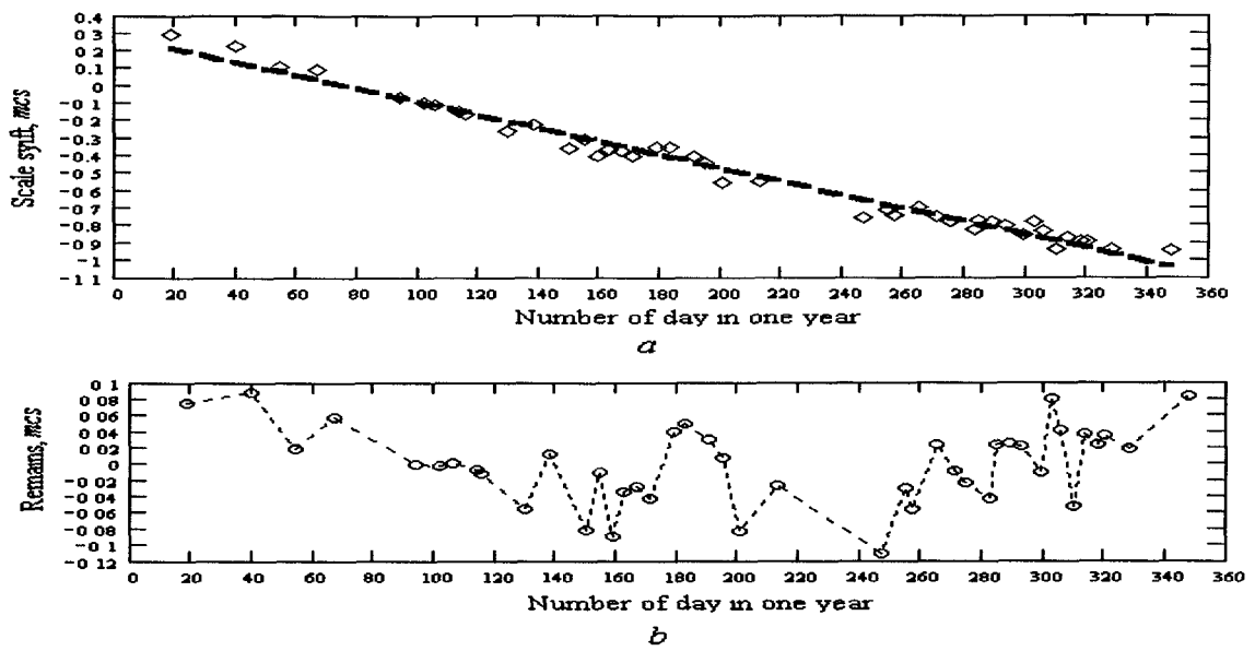
Figure 4. Outcomes of the regression analysis for the first-order model.
