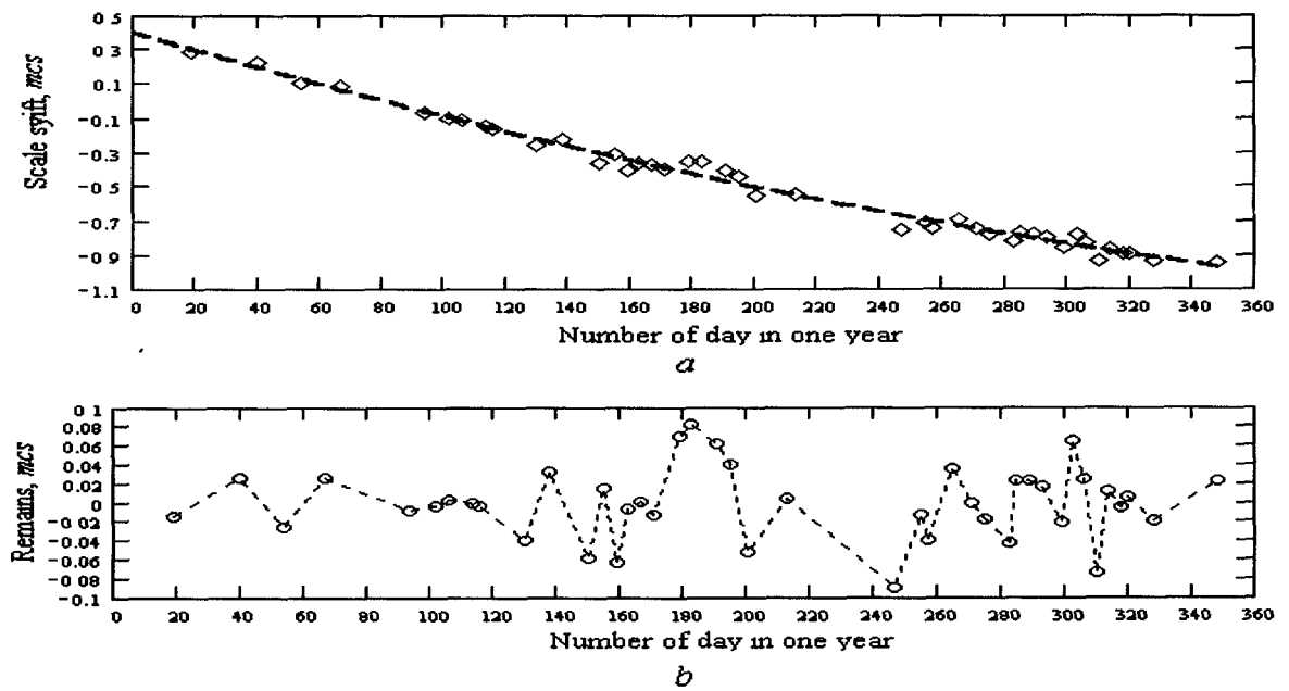
Figure 5. Outcomes of the regression analysis for the second-order model.
