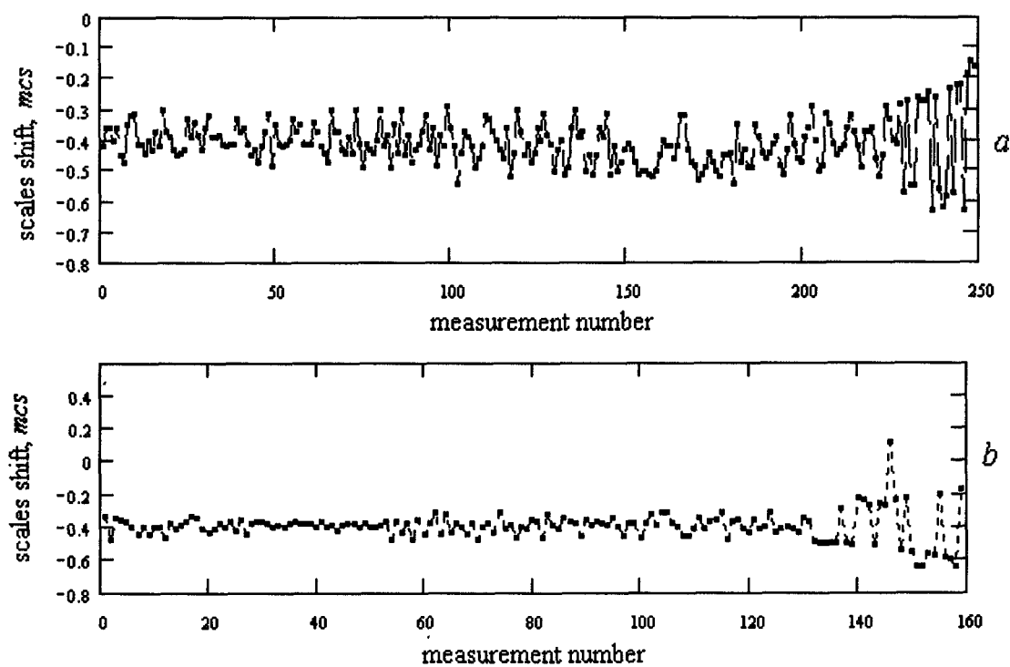
Figure 3. Examples of realizations from long meteoric tracks.
