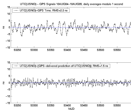
Figure 2. Recent daily averages of UTC (USNO) minus GPS Time and UTC minus GPS's delivered prediction of UTC (USNO).
