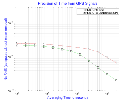
Figure 3. The precision of GPS Time and of GPS's delivered prediction of UTC (USNO), using 3 years of TTR-12 data, measured by the attainable external precision (rms, mean not removed) as a function of averaging time, and referenced to UTC (USNO). Improved performance in accessing UTC (USNO) could be realized if only the most recently updated navigation messages are used. The accuracy attainable over a given averaging time also depends upon the calibration of the user's receivers.
