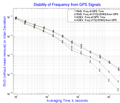
Figure 4. RMS frequency external precision and the frequency stability, as measured by the Allan deviation, of GPS Time and for GPS's delivered prediction of UTC (USNO), using TTR-12 data from 11JUL02 to 12AUG05. Reference frequency is that of UTC (USNO).
