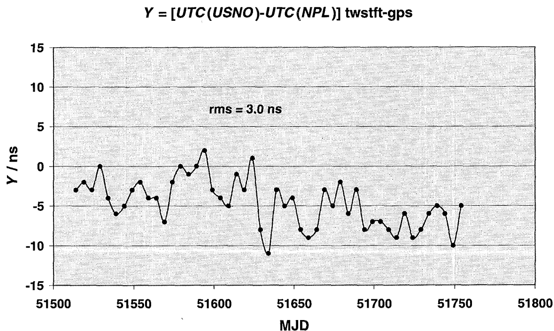
Figure 8. Differences between TWSTFT and GPS common-view for USNO/NPL link.
