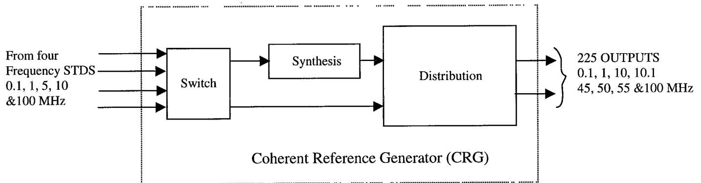
Figure 2. Reference Frequency Synthesis and Distribution
